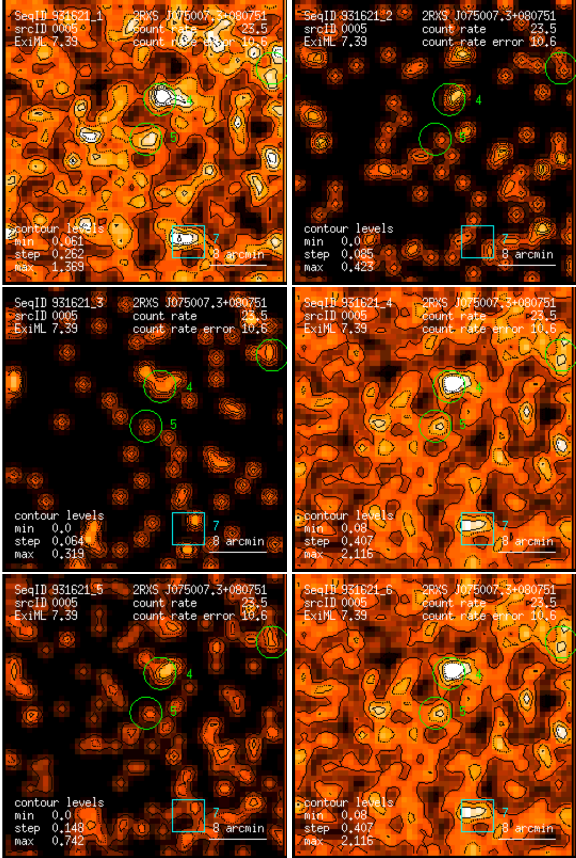
Figure 5: RASS 931621: detection 0005: band rate images, Gaussian filter: (1) PSPC channels 11 – 41, (2) 52 – 90, (3) 91 – 201, (4) 11 – 235, (5) 52 – 201, (6) 11 – 201. Broad band rates in counts/ks. Band rate contour levels in counts/ks/arcmin 2 .
