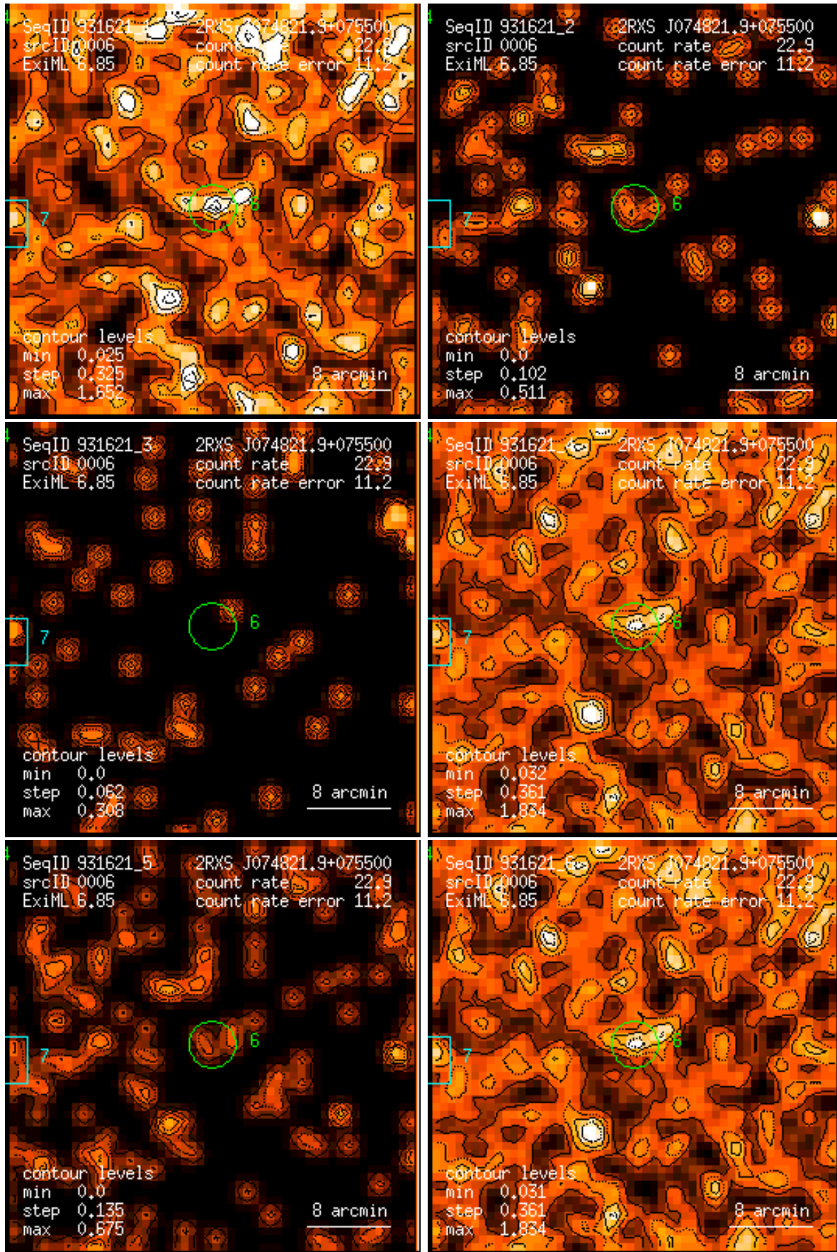
Figure 6: RASS 931621: detection 0006: band rate images, Gaussian filter: (1) PSPC channels 11 – 41, (2) 52 – 90, (3) 91 – 201, (4) 11 – 235, (5) 52 – 201, (6) 11 – 201. Broad band rates in counts/ks. Band rate contour levels in counts/ks/arcmin 2 .
