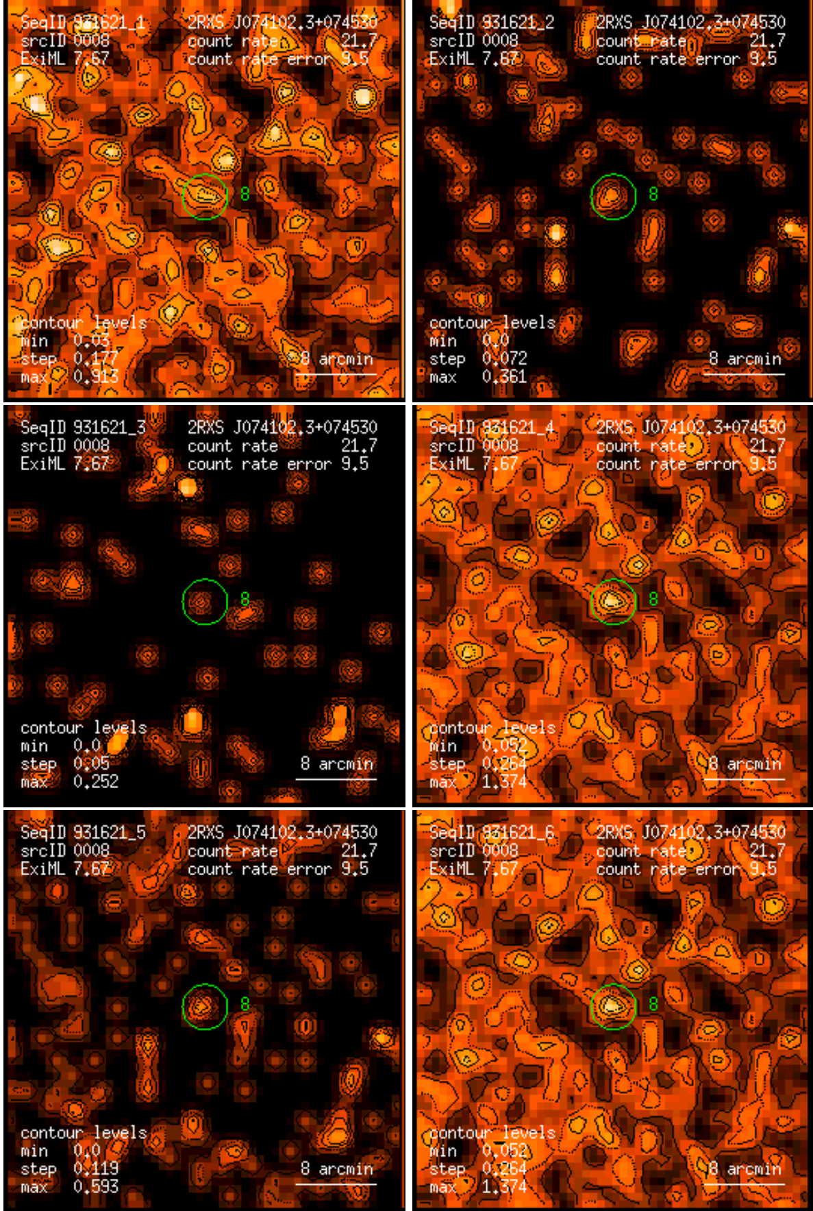
Figure 8: RASS 931621: detection 0008: band rate images, Gaussian filter: (1) PSPC channels 11 – 41, (2) 52 – 90, (3) 91 – 201, (4) 11 – 235, (5) 52 – 201, (6) 11 – 201. Broad band rates in counts/ks. Band rate contour levels in counts/ks/arcmin 2 .
