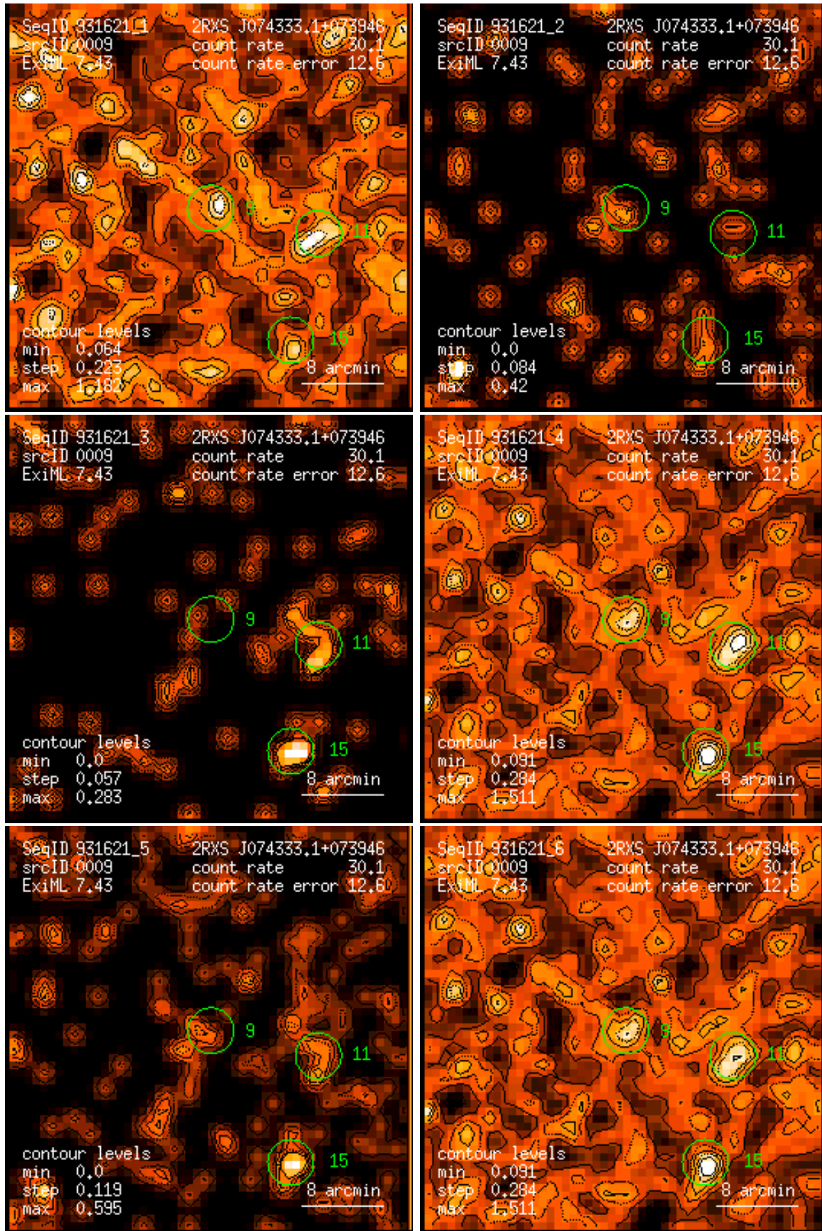
Figure 9: RASS 931621: detection 0009: band rate images, Gaussian filter: (1) PSPC channels 11 – 41, (2) 52 – 90, (3) 91 – 201, (4) 11 – 235, (5) 52 – 201, (6) 11 – 201. Broad band rates in counts/ks. Band rate contour levels in counts/ks/arcmin 2 .
