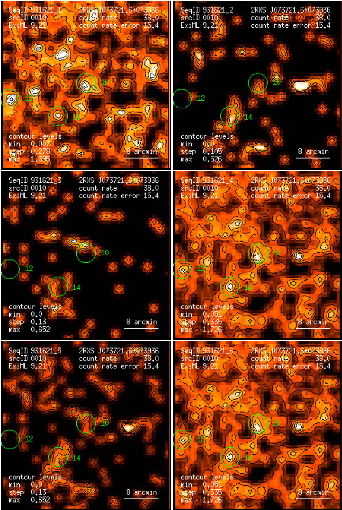
Figure 10: RASS 931621: detection 0010: band rate images, Gaussian filter: (1) PSPC channels 11 – 41, (2) 52 – 90, (3) 91 – 201, (4) 11 – 235, (5) 52 – 201, (6) 11 – 201. Broad band rates in counts/ks. Band rate contour levels in counts/ks/arcmin 2 .
