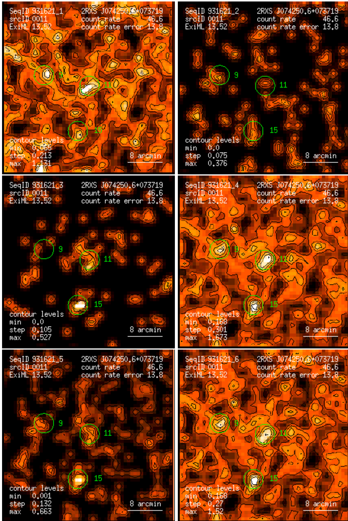
Figure 11: RASS 931621: detection 0011: band rate images, Gaussian filter: (1) PSPC channels 11 – 41, (2) 52 – 90, (3) 91 – 201, (4) 11 – 235, (5) 52 – 201, (6) 11 – 201. Broad band rates in counts/ks. Band rate contour levels in counts/ks/arcmin 2 .
