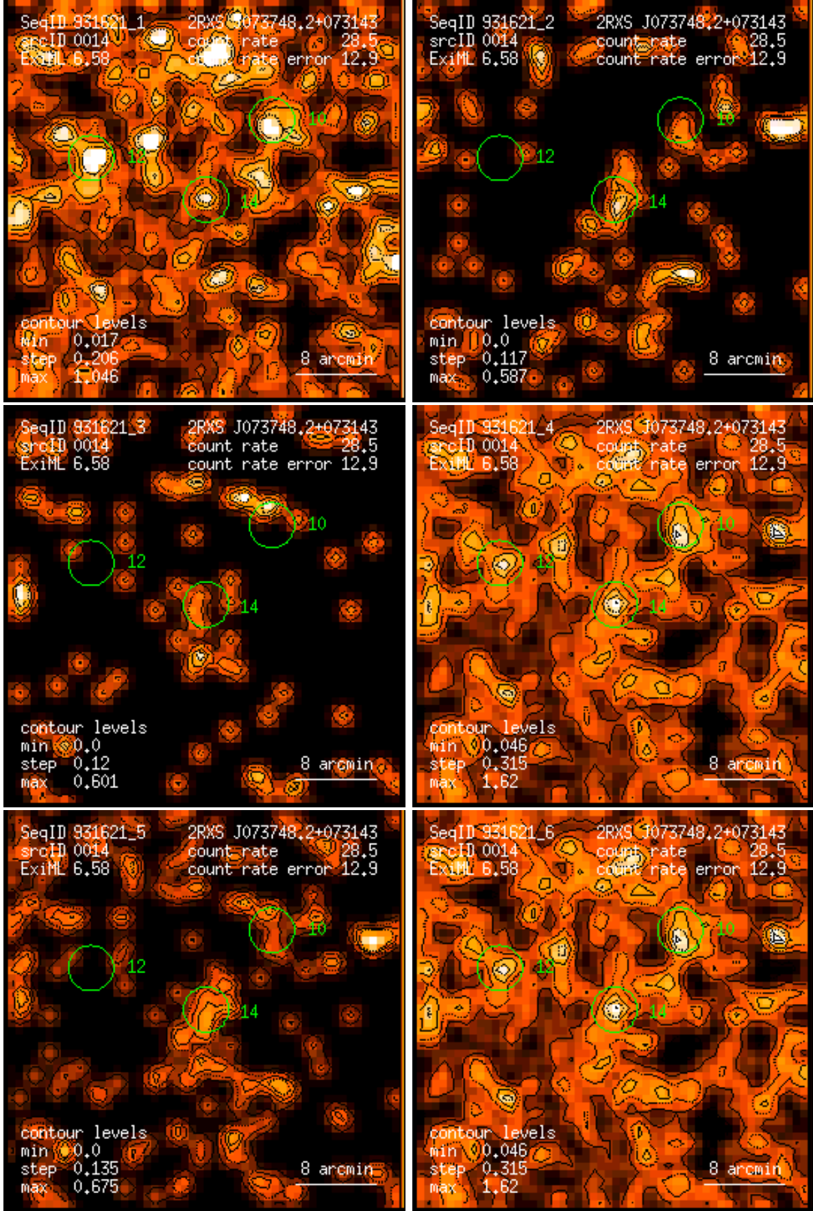
Figure 14: RASS 931621: detection 0014: band rate images, Gaussian filter: (1) PSPC channels 11 – 41, (2) 52 – 90, (3) 91 – 201, (4) 11 – 235, (5) 52 – 201, (6) 11 – 201. Broad band rates in counts/ks. Band rate contour levels in counts/ks/arcmin 2 .
