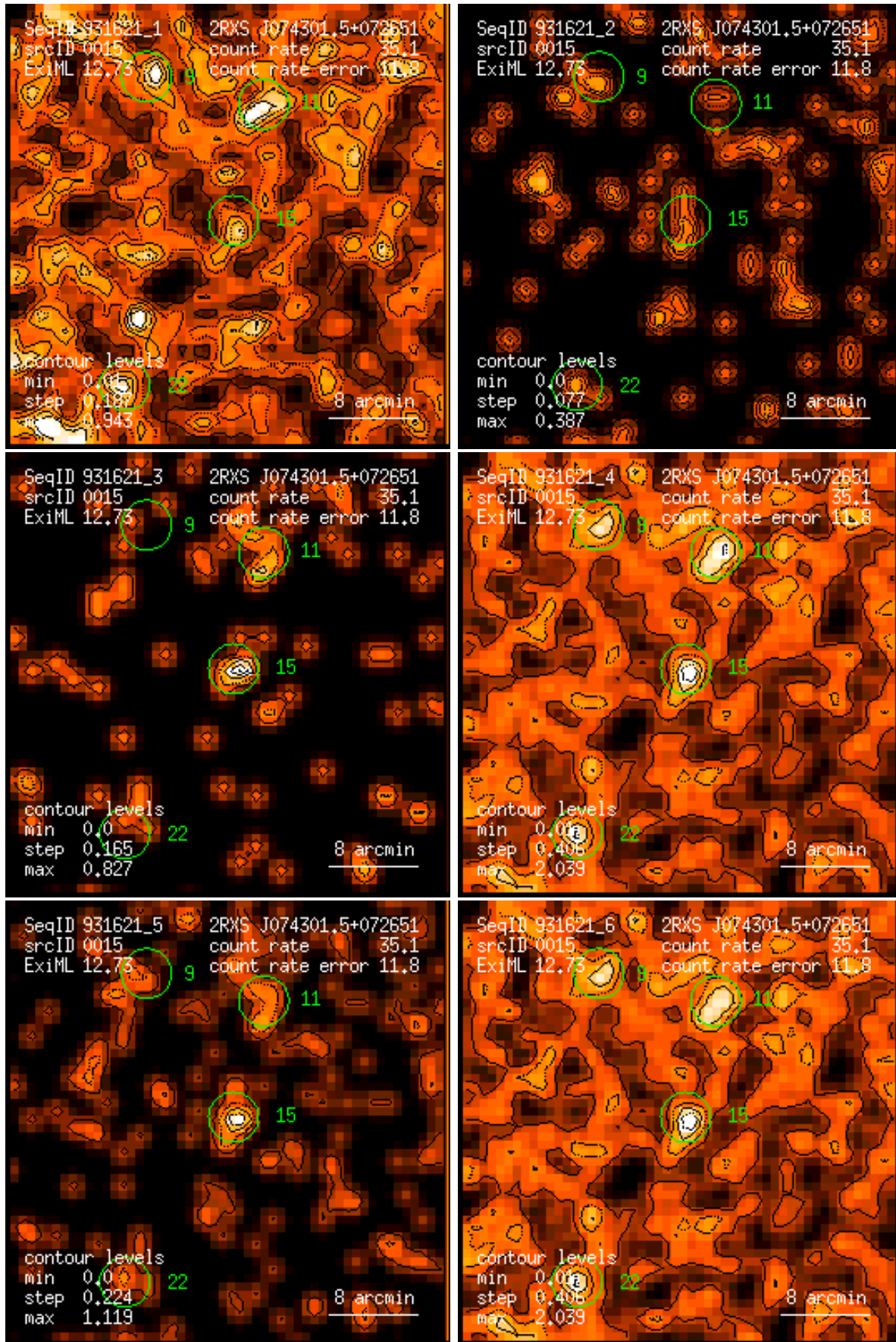
Figure 15: RASS 931621: detection 0015: band rate images, Gaussian filter: (1) PSPC channels 11 – 41, (2) 52 – 90, (3) 91 – 201, (4) 11 – 235, (5) 52 – 201, (6) 11 – 201. Broad band rates in counts/ks. Band rate contour levels in counts/ks/arcmin 2 .
