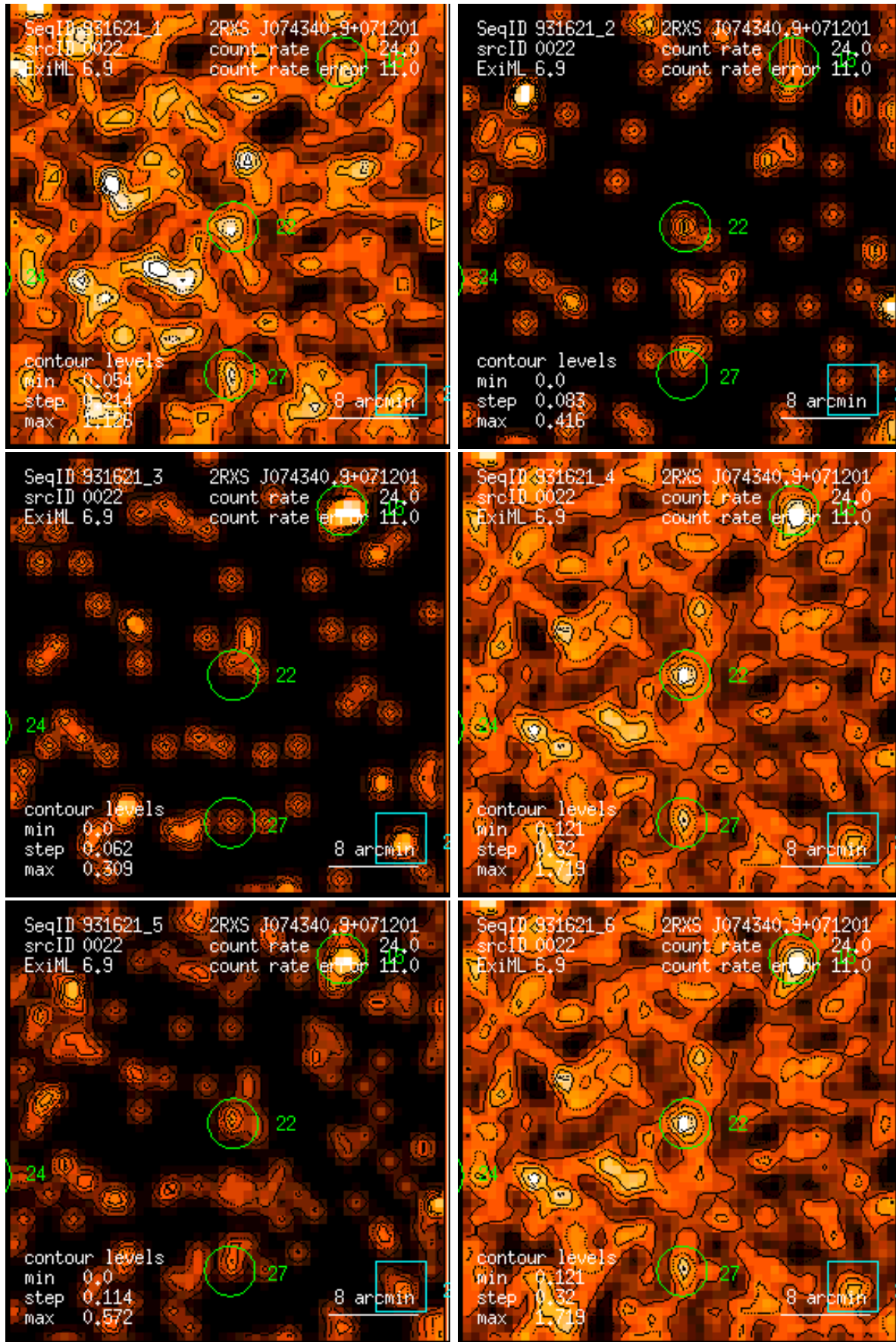
Figure 22: RASS 931621: detection 0022: band rate images, Gaussian filter: (1) PSPC channels 11 – 41, (2) 52 – 90, (3) 91 – 201, (4) 11 – 235, (5) 52 – 201, (6) 11 – 201. Broad band rates in counts/ks. Band rate contour levels in counts/ks/arcmin 2 .
