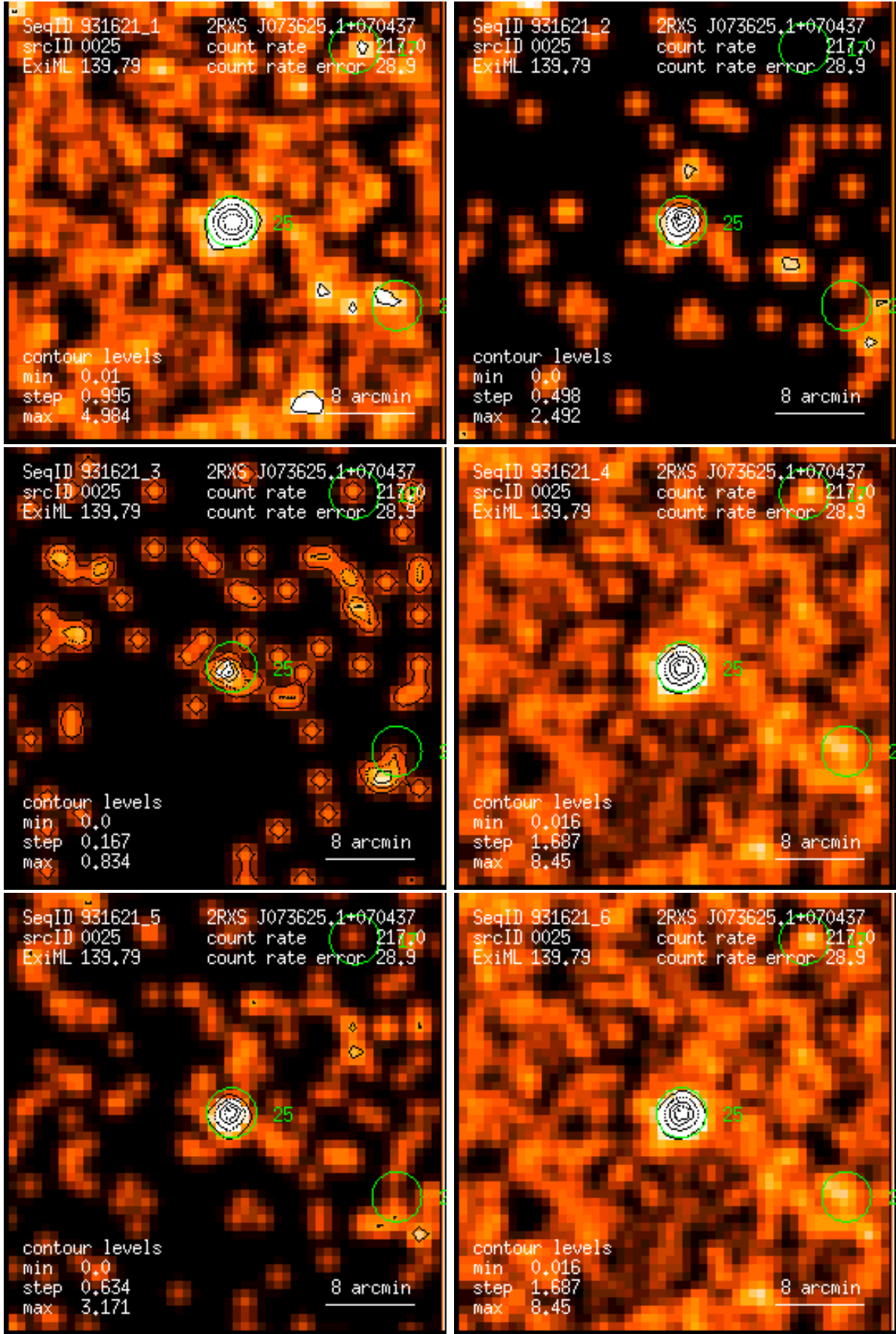
Figure 25: RASS 931621: detection 0025: band rate images, Gaussian filter: (1) PSPC channels 11 – 41, (2) 52 – 90, (3) 91 – 201, (4) 11 – 235, (5) 52 – 201, (6) 11 – 201. Broad band rates in counts/ks. Band rate contour levels in counts/ks/arcmin 2 .
