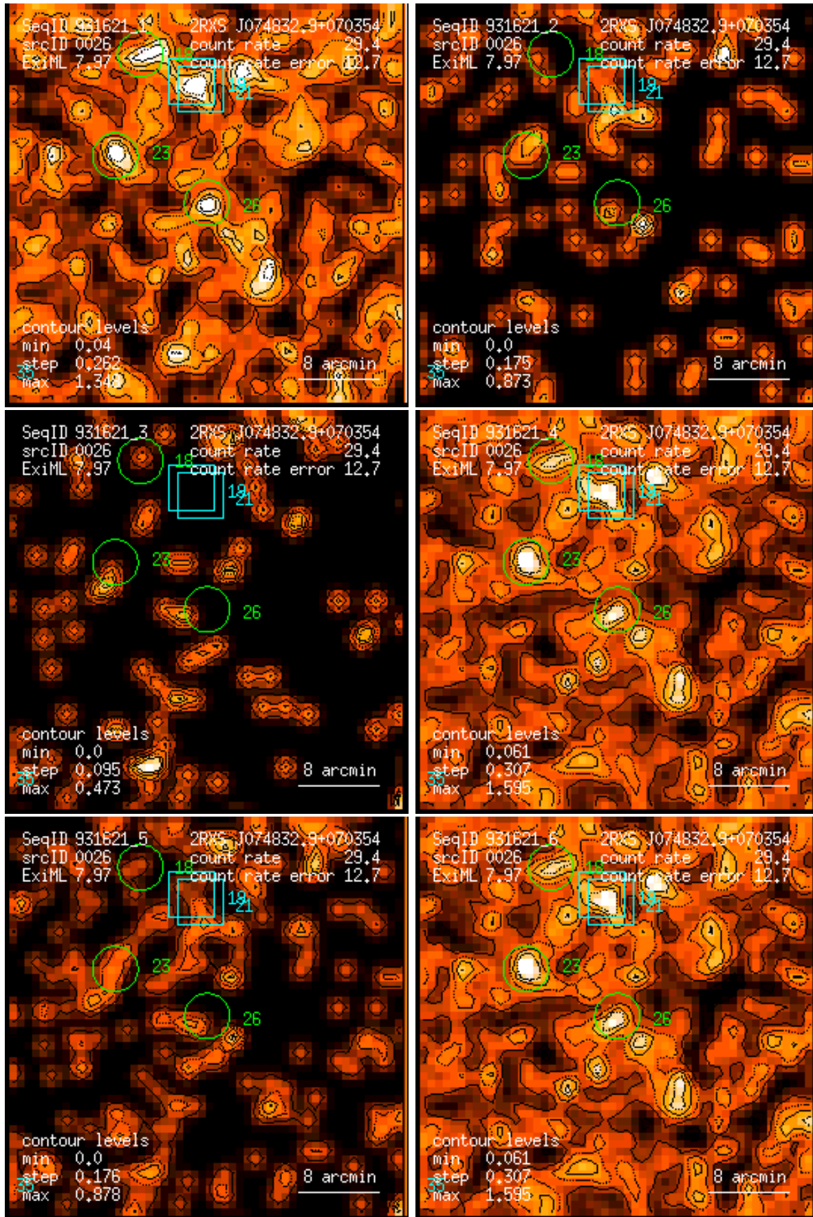
Figure 26: RASS 931621: detection 0026: band rate images, Gaussian filter: (1) PSPC channels 11 – 41, (2) 52 – 90, (3) 91 – 201, (4) 11 – 235, (5) 52 – 201, (6) 11 – 201. Broad band rates in counts/ks. Band rate contour levels in counts/ks/arcmin 2 .
