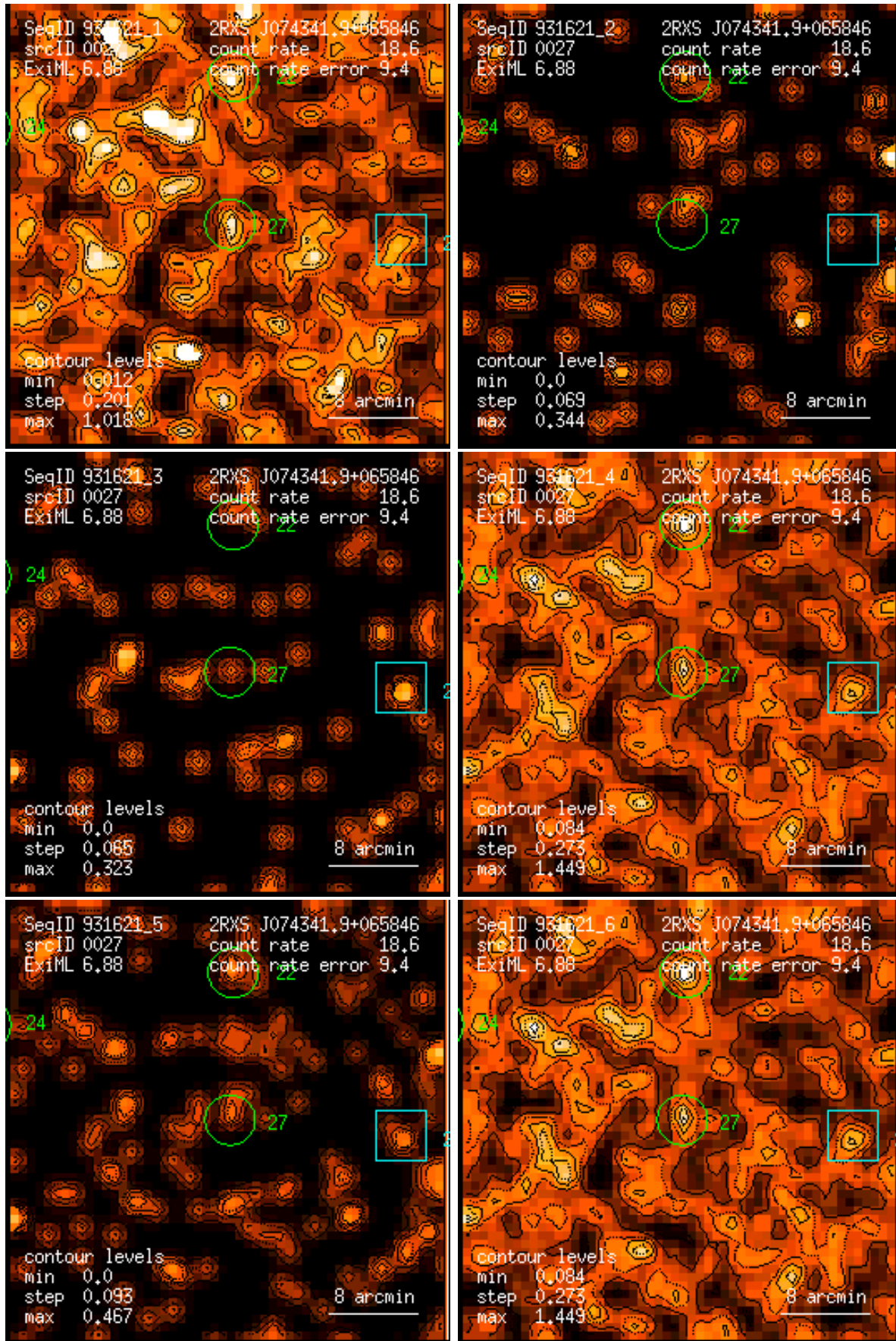
Figure 27: RASS 931621: detection 0027: band rate images, Gaussian filter: (1) PSPC channels 11 – 41, (2) 52 – 90, (3) 91 – 201, (4) 11 – 235, (5) 52 – 201, (6) 11 – 201. Broad band rates in counts/ks. Band rate contour levels in counts/ks/arcmin 2 .
