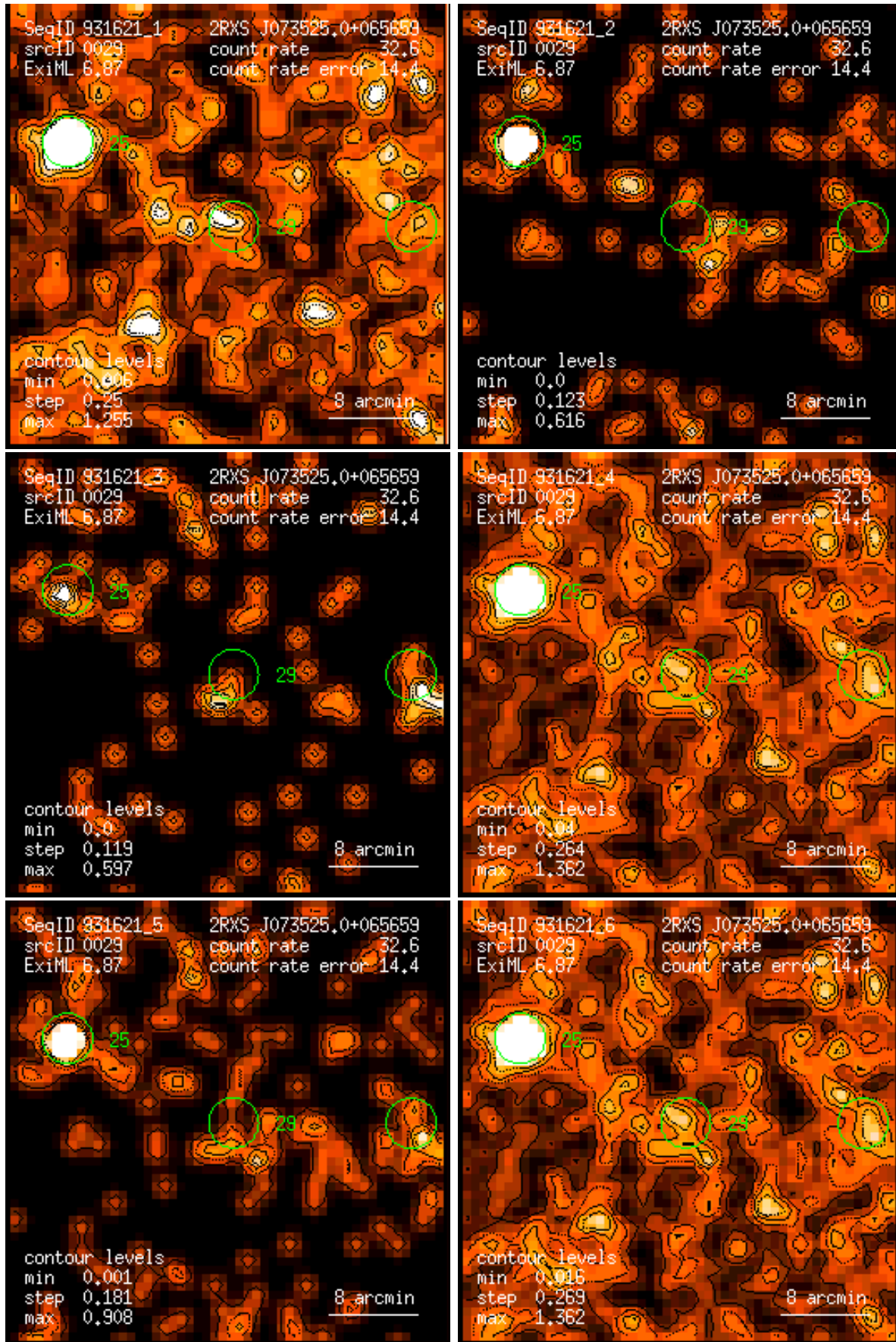
Figure 29: RASS 931621: detection 0029: band rate images, Gaussian filter: (1) PSPC channels 11 – 41, (2) 52 – 90, (3) 91 – 201, (4) 11 – 235, (5) 52 – 201, (6) 11 – 201. Broad band rates in counts/ks. Band rate contour levels in counts/ks/arcmin 2 .
