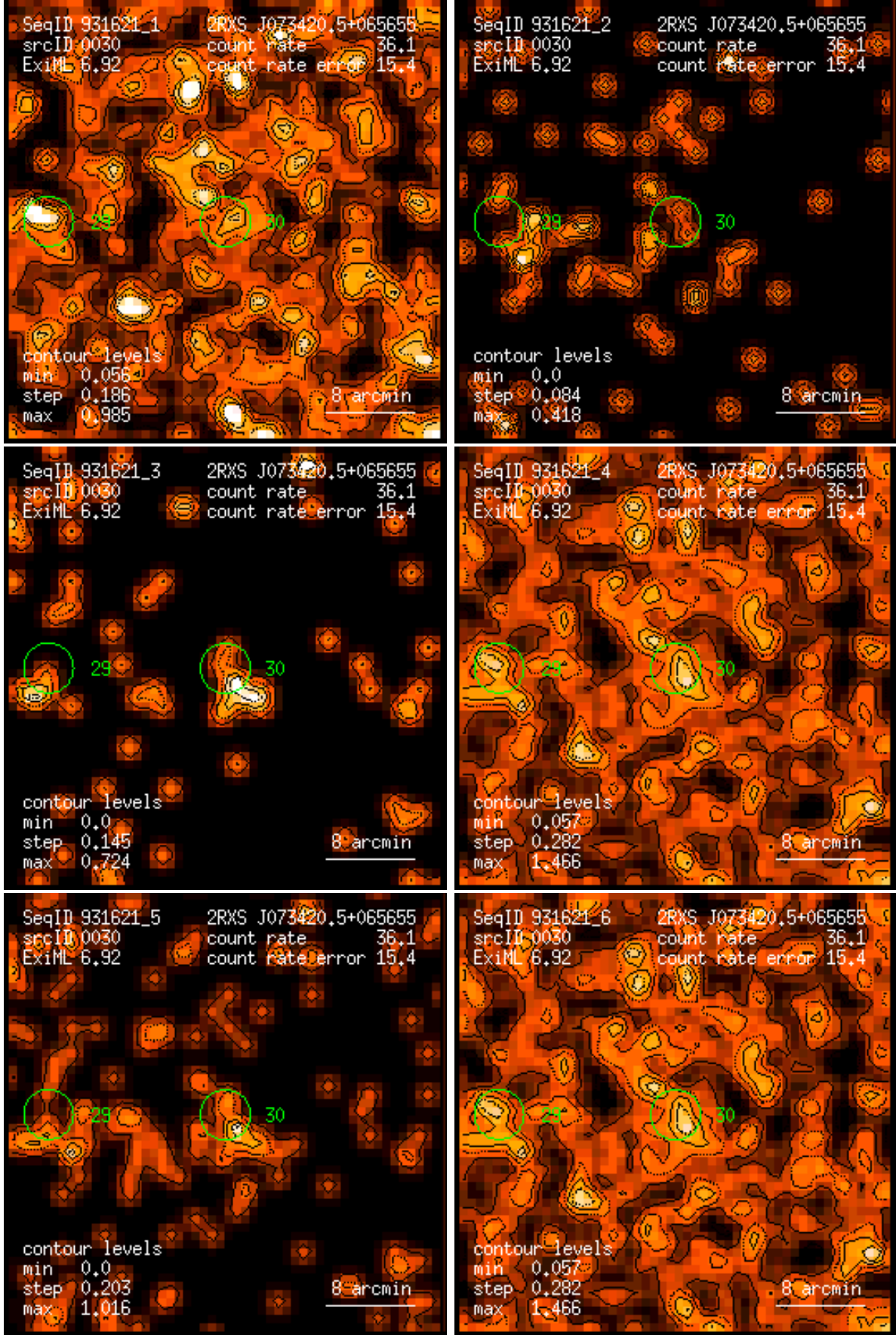
Figure 30: RASS 931621: detection 0030: band rate images, Gaussian filter: (1) PSPC channels 11 – 41, (2) 52 – 90, (3) 91 – 201, (4) 11 – 235, (5) 52 – 201, (6) 11 – 201. Broad band rates in counts/ks. Band rate contour levels in counts/ks/arcmin 2 .
