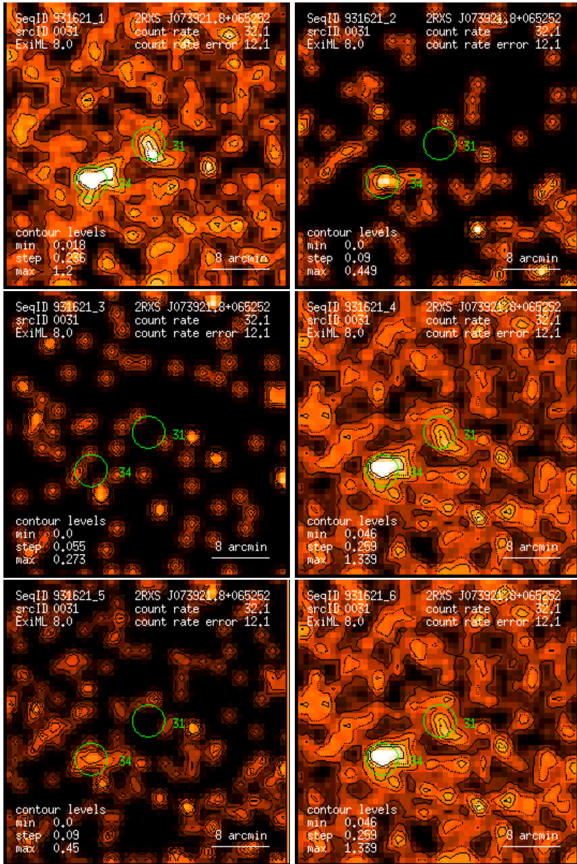
Figure 31: RASS 931621: detection 0031: band rate images, Gaussian filter: (1) PSPC channels 11 – 41, (2) 52 – 90, (3) 91 – 201, (4) 11 – 235, (5) 52 – 201, (6) 11 – 201. Broad band rates in counts/ks. Band rate contour levels in counts/ks/arcmin 2 .
