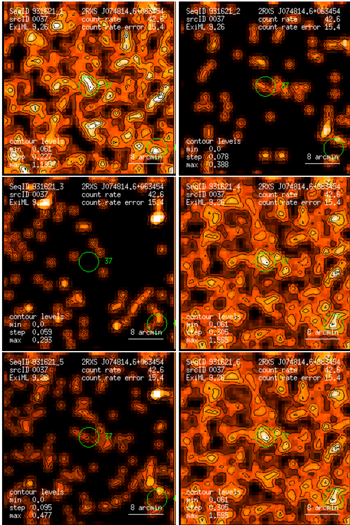
Figure 37: RASS 931621: detection 0037: band rate images, Gaussian filter: (1) PSPC channels 11 – 41, (2) 52 – 90, (3) 91 – 201, (4) 11 – 235, (5) 52 – 201, (6) 11 – 201. Broad band rates in counts/ks. Band rate contour levels in counts/ks/arcmin 2 .
