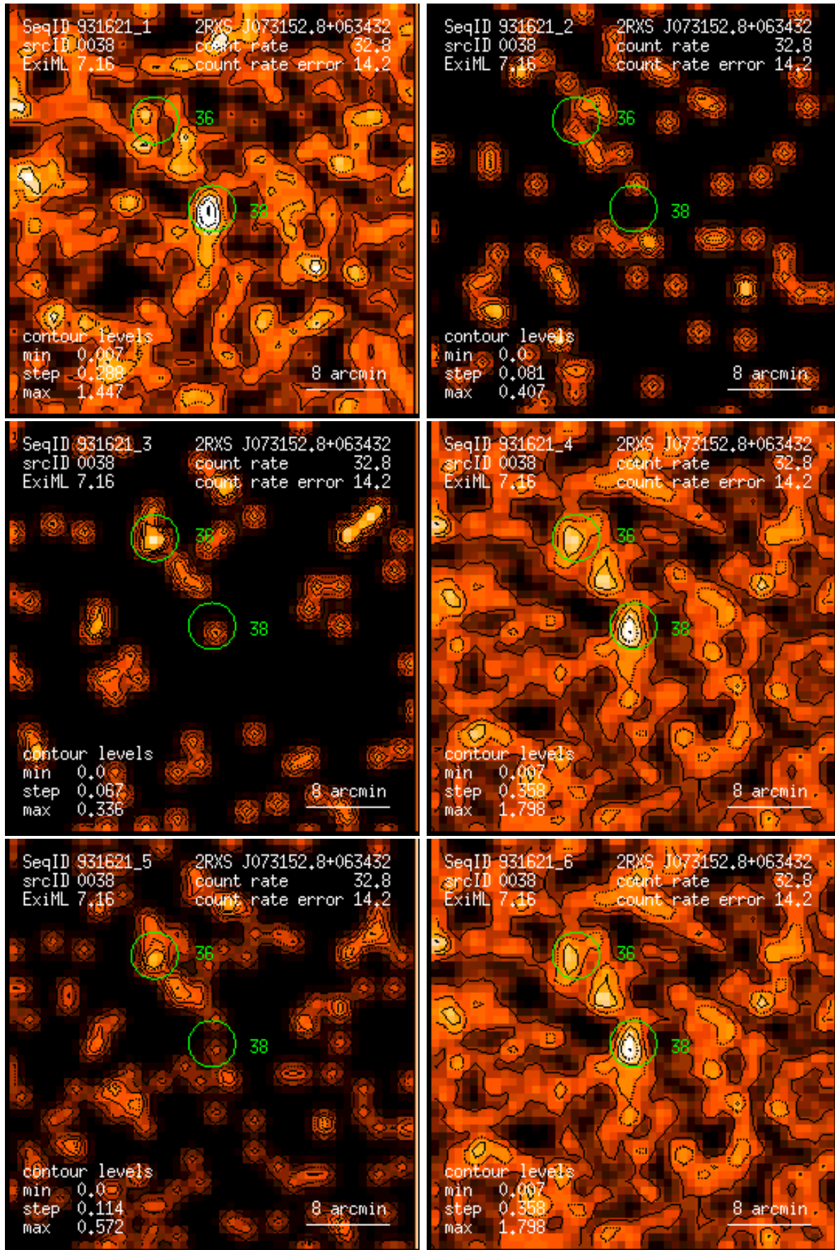
Figure 38: RASS 931621: detection 0038: band rate images, Gaussian filter: (1) PSPC channels 11 – 41, (2) 52 – 90, (3) 91 – 201, (4) 11 – 235, (5) 52 – 201, (6) 11 – 201. Broad band rates in counts/ks. Band rate contour levels in counts/ks/arcmin 2 .
