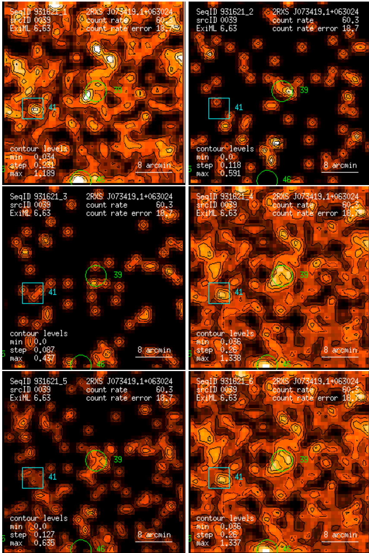
Figure 39: RASS 931621: detection 0039: band rate images, Gaussian filter: (1) PSPC channels 11 – 41, (2) 52 – 90, (3) 91 – 201, (4) 11 – 235, (5) 52 – 201, (6) 11 – 201. Broad band rates in counts/ks. Band rate contour levels in counts/ks/arcmin 2 .
