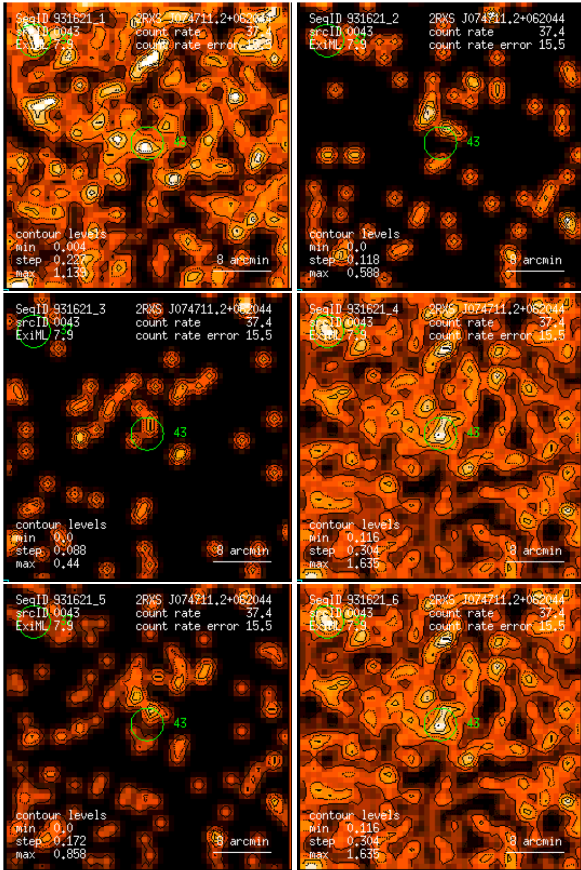
Figure 43: RASS 931621: detection 0043: band rate images, Gaussian filter: (1) PSPC channels 11 – 41, (2) 52 – 90, (3) 91 – 201, (4) 11 – 235, (5) 52 – 201, (6) 11 – 201. Broad band rates in counts/ks. Band rate contour levels in counts/ks/arcmin 2 .
