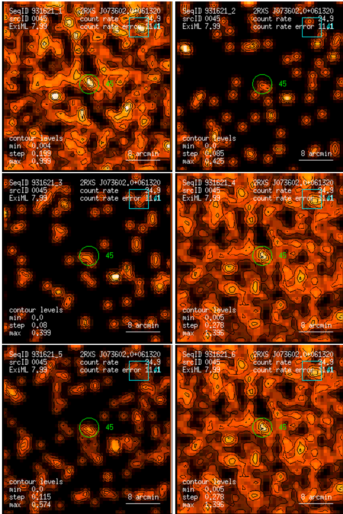
Figure 45: RASS 931621: detection 0045: band rate images, Gaussian filter: (1) PSPC channels 11 – 41, (2) 52 – 90, (3) 91 – 201, (4) 11 – 235, (5) 52 – 201, (6) 11 – 201. Broad band rates in counts/ks. Band rate contour levels in counts/ks/arcmin 2 .
