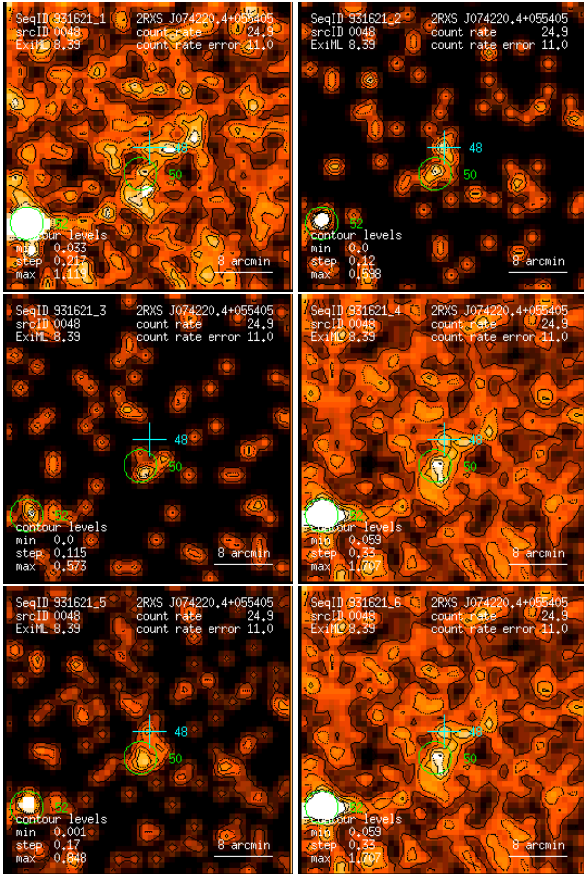
Figure 48: RASS 931621: detection 0048: band rate images, Gaussian filter: (1) PSPC channels 11 – 41, (2) 52 – 90, (3) 91 – 201, (4) 11 – 235, (5) 52 – 201, (6) 11 – 201. Broad band rates in counts/ks. Band rate contour levels in counts/ks/arcmin 2 .
