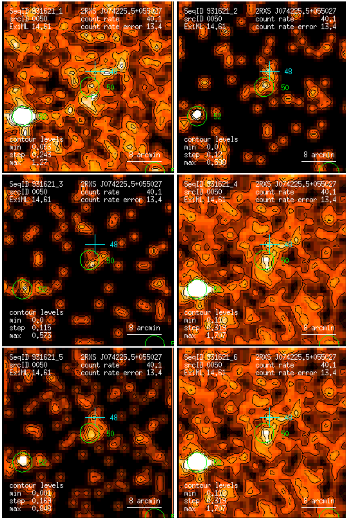
Figure 50: RASS 931621: detection 0050: band rate images, Gaussian filter: (1) PSPC channels 11 – 41, (2) 52 – 90, (3) 91 – 201, (4) 11 – 235, (5) 52 – 201, (6) 11 – 201. Broad band rates in counts/ks. Band rate contour levels in counts/ks/arcmin 2 .
