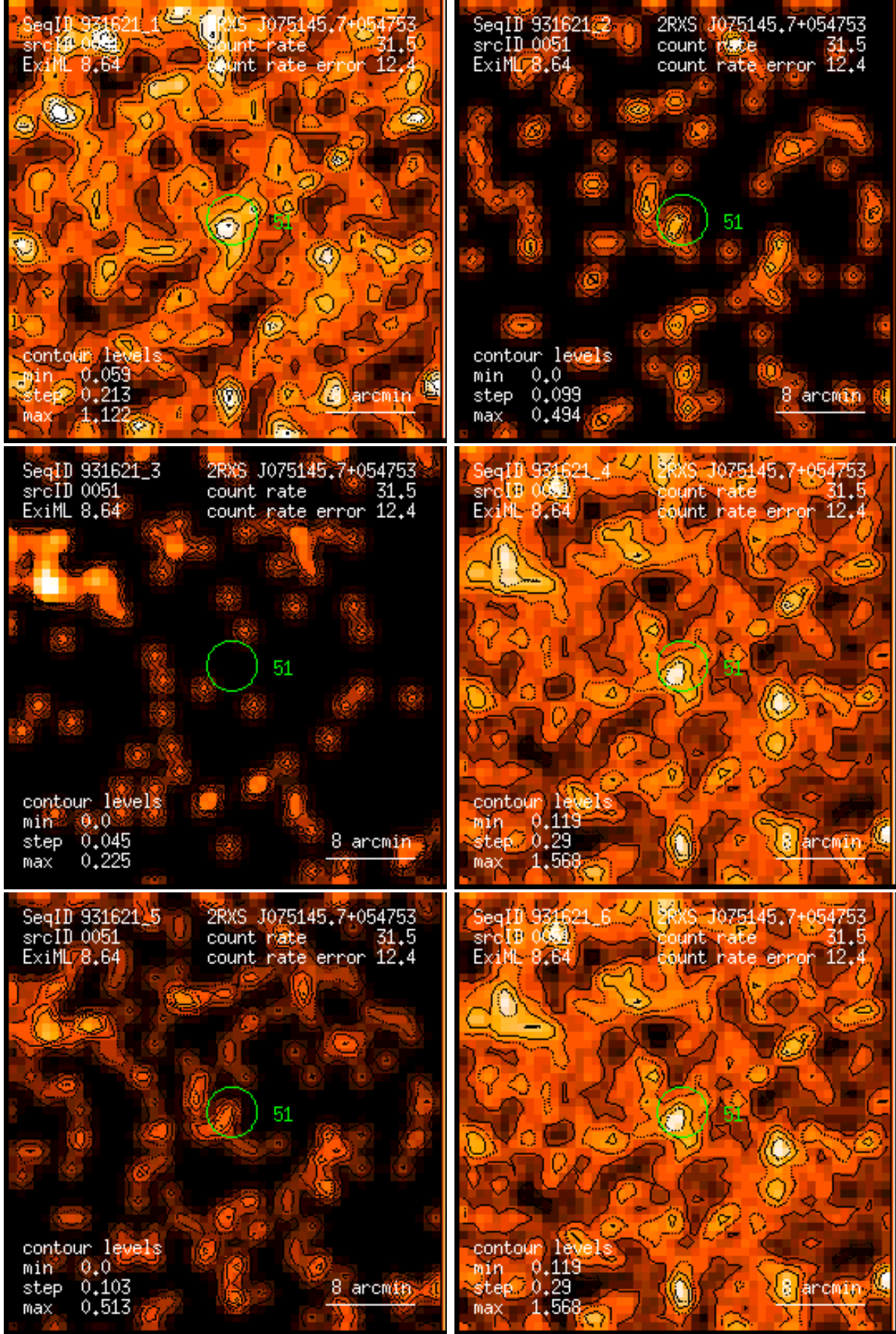
Figure 51: RASS 931621: detection 0051: band rate images, Gaussian filter: (1) PSPC channels 11 – 41, (2) 52 – 90, (3) 91 – 201, (4) 11 – 235, (5) 52 – 201, (6) 11 – 201. Broad band rates in counts/ks. Band rate contour levels in counts/ks/arcmin 2 .
