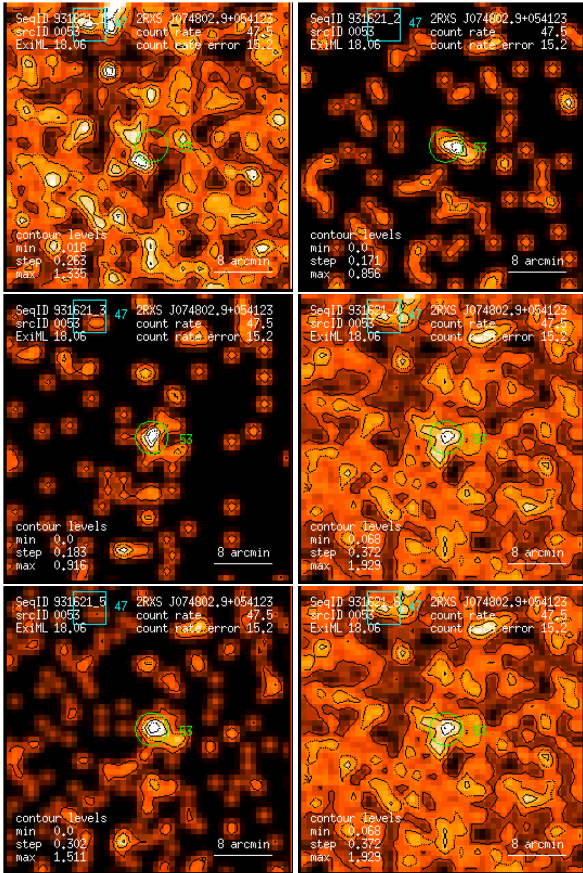
Figure 53: RASS 931621: detection 0053: band rate images, Gaussian filter: (1) PSPC channels 11 – 41, (2) 52 – 90, (3) 91 – 201, (4) 11 – 235, (5) 52 – 201, (6) 11 – 201. Broad band rates in counts/ks. Band rate contour levels in counts/ks/arcmin 2 .
