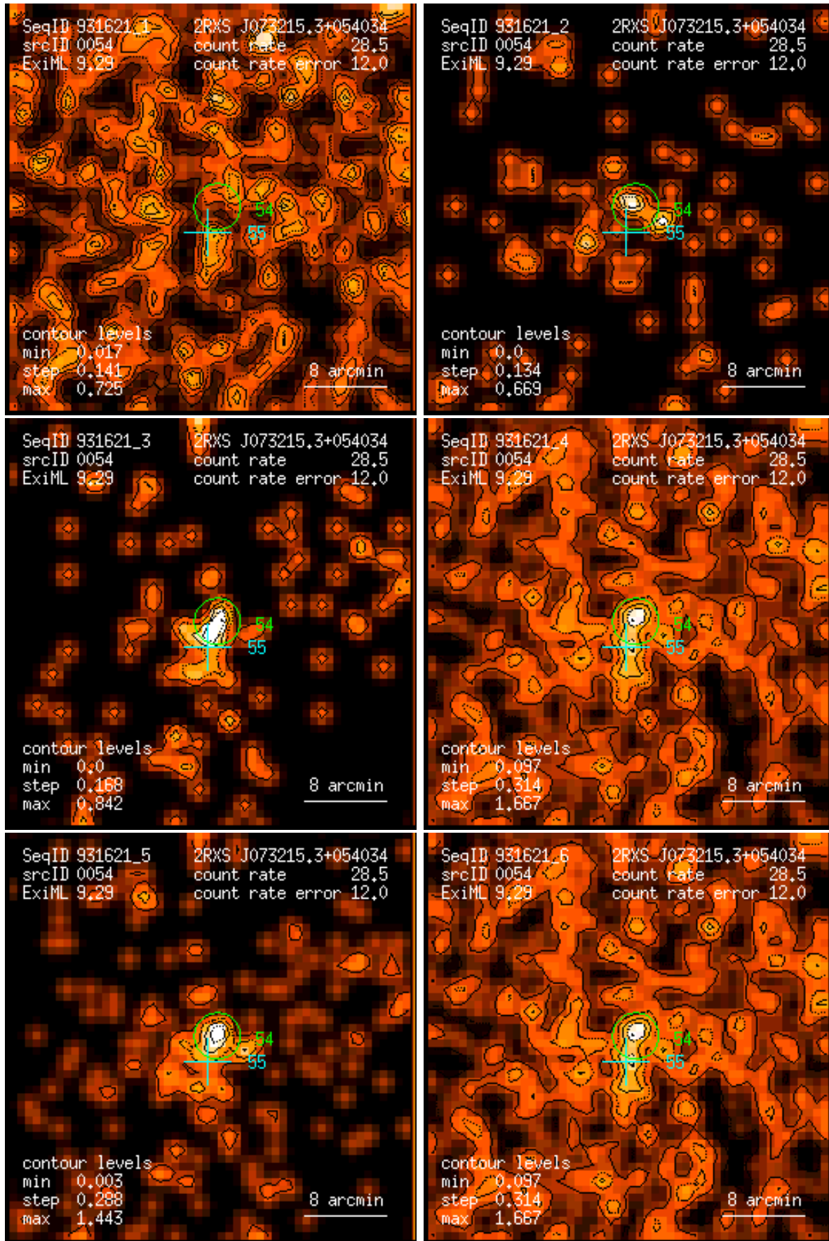
Figure 54: RASS 931621: detection 0054: band rate images, Gaussian filter: (1) PSPC channels 11 – 41, (2) 52 – 90, (3) 91 – 201, (4) 11 – 235, (5) 52 – 201, (6) 11 – 201. Broad band rates in counts/ks. Band rate contour levels in counts/ks/arcmin 2 .
