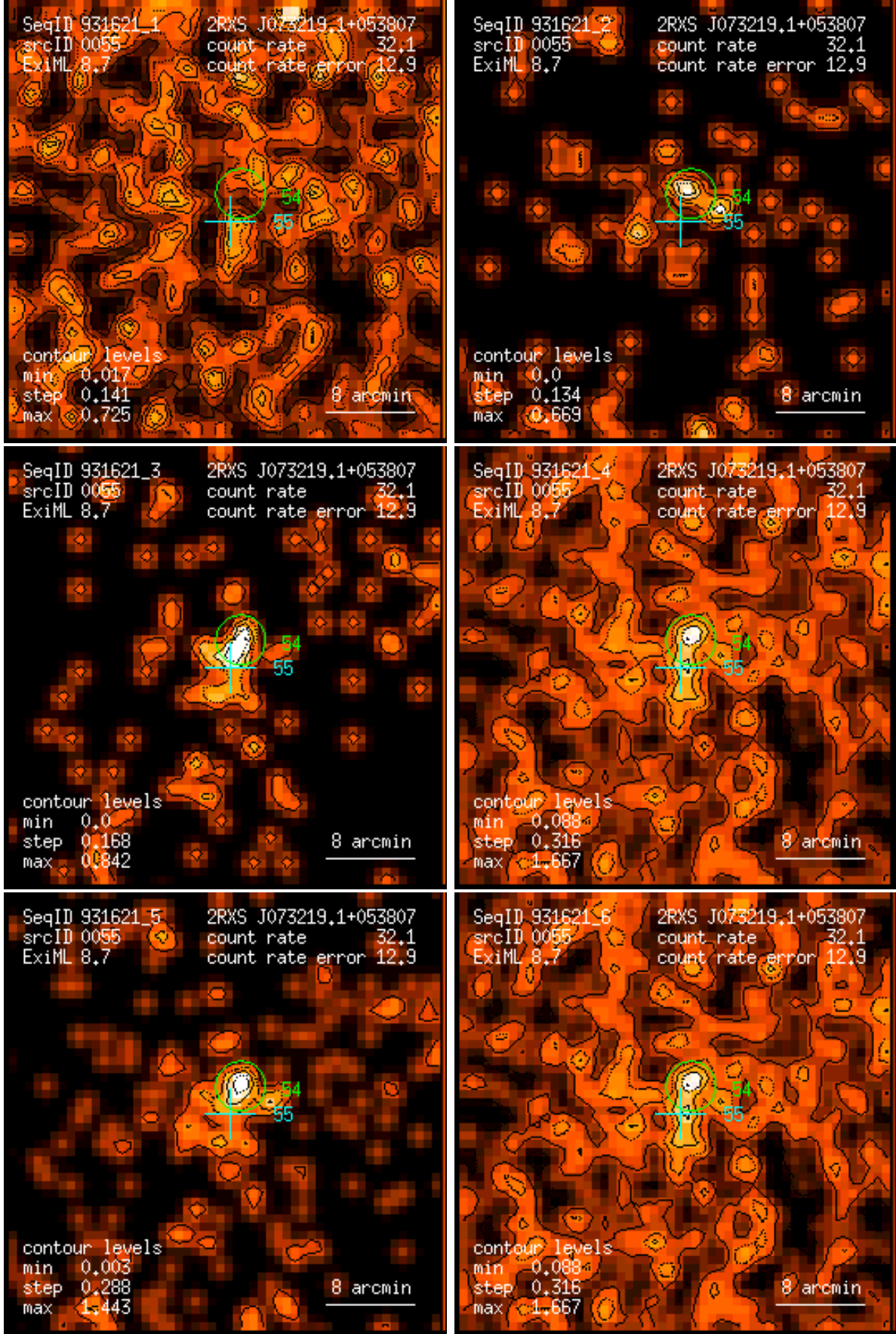
Figure 55: RASS 931621: detection 0055: band rate images, Gaussian filter: (1) PSPC channels 11 – 41, (2) 52 – 90, (3) 91 – 201, (4) 11 – 235, (5) 52 – 201, (6) 11 – 201. Broad band rates in counts/ks. Band rate contour levels in counts/ks/arcmin 2 .
