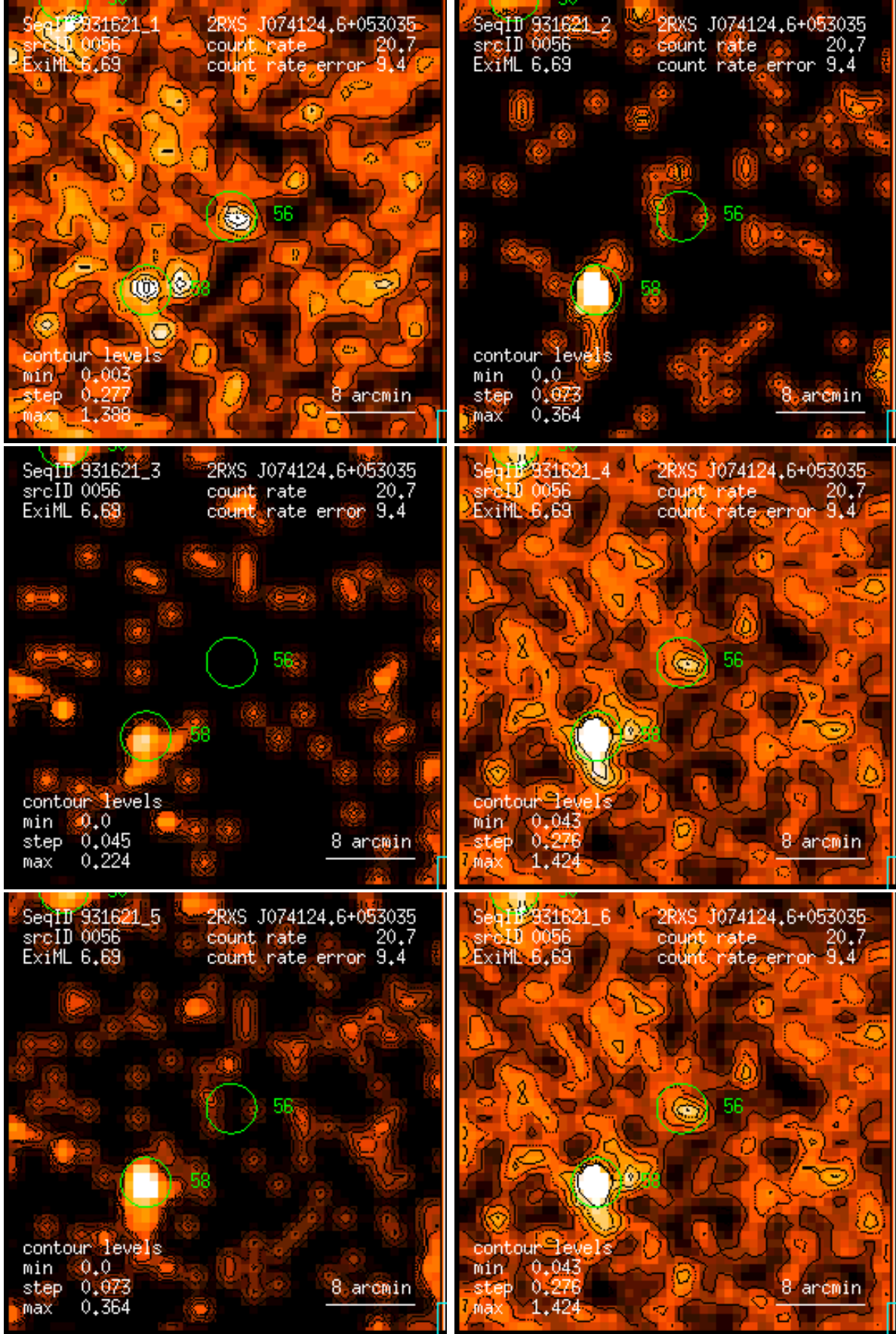
Figure 56: RASS 931621: detection 0056: band rate images, Gaussian filter: (1) PSPC channels 11 – 41, (2) 52 – 90, (3) 91 – 201, (4) 11 – 235, (5) 52 – 201, (6) 11 – 201. Broad band rates in counts/ks. Band rate contour levels in counts/ks/arcmin 2 .
