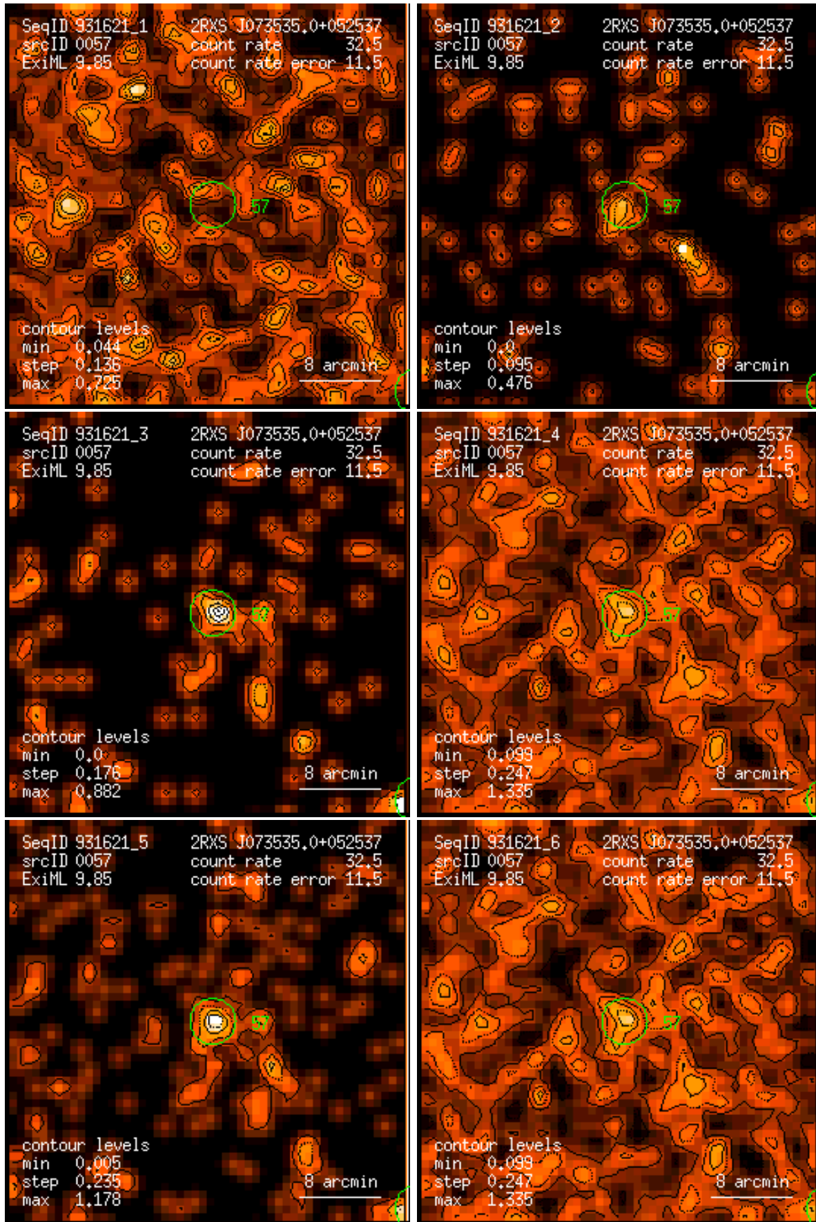
Figure 57: RASS 931621: detection 0057: band rate images, Gaussian filter: (1) PSPC channels 11 – 41, (2) 52 – 90, (3) 91 – 201, (4) 11 – 235, (5) 52 – 201, (6) 11 – 201. Broad band rates in counts/ks. Band rate contour levels in counts/ks/arcmin 2 .
