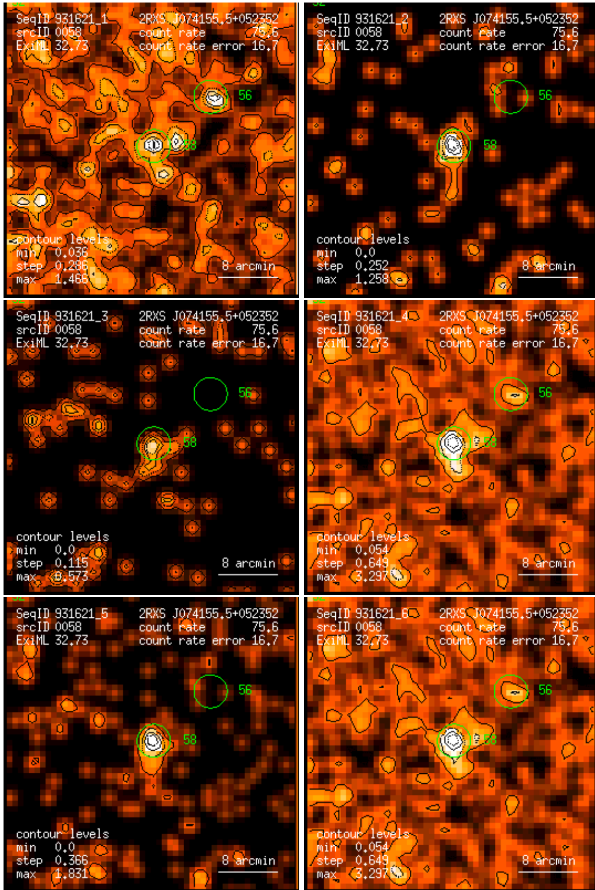
Figure 58: RASS 931621: detection 0058: band rate images, Gaussian filter: (1) PSPC channels 11 – 41, (2) 52 – 90, (3) 91 – 201, (4) 11 – 235, (5) 52 – 201, (6) 11 – 201. Broad band rates in counts/ks. Band rate contour levels in counts/ks/arcmin 2 .
