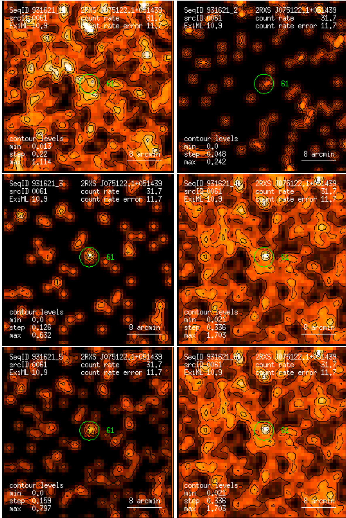
Figure 61: RASS 931621: detection 0061: band rate images, Gaussian filter: (1) PSPC channels 11 – 41, (2) 52 – 90, (3) 91 – 201, (4) 11 – 235, (5) 52 – 201, (6) 11 – 201. Broad band rates in counts/ks. Band rate contour levels in counts/ks/arcmin 2 .
