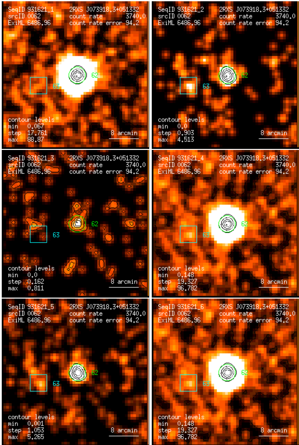
Figure 62: RASS 931621: detection 0062: band rate images, Gaussian filter: (1) PSPC channels 11 – 41, (2) 52 – 90, (3) 91 – 201, (4) 11 – 235, (5) 52 – 201, (6) 11 – 201. Broad band rates in counts/ks. Band rate contour levels in counts/ks/arcmin 2 .
