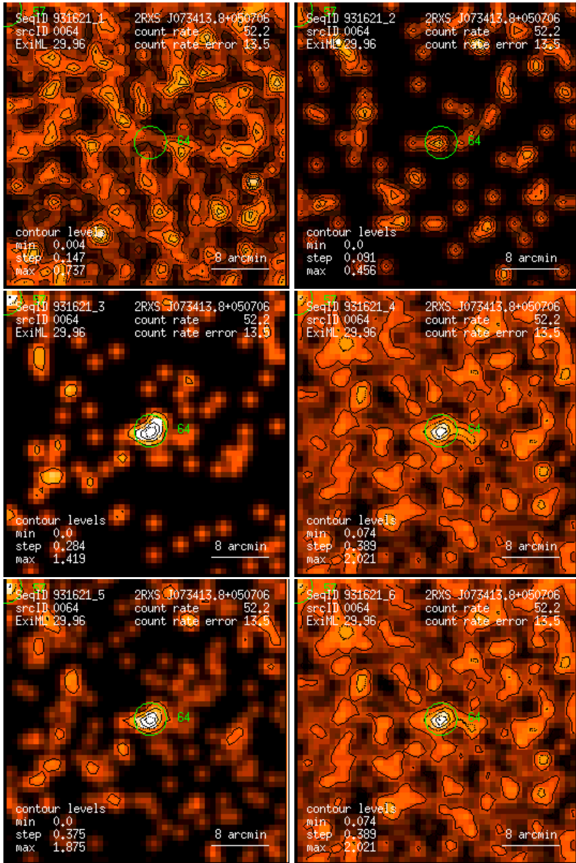
Figure 64: RASS 931621: detection 0064: band rate images, Gaussian filter: (1) PSPC channels 11 – 41, (2) 52 – 90, (3) 91 – 201, (4) 11 – 235, (5) 52 – 201, (6) 11 – 201. Broad band rates in counts/ks. Band rate contour levels in counts/ks/arcmin 2 .
