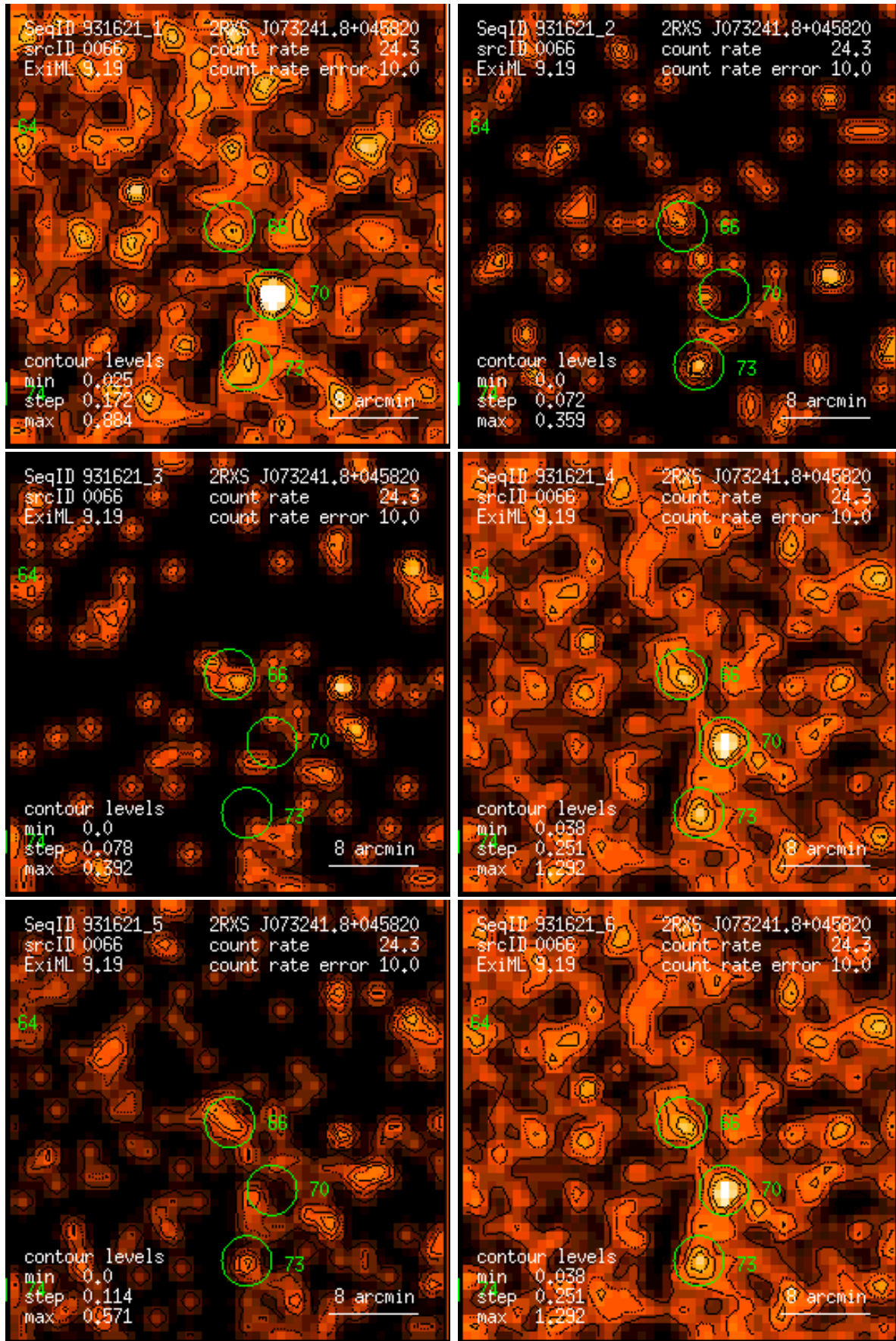
Figure 66: RASS 931621: detection 0066: band rate images, Gaussian filter: (1) PSPC channels 11 – 41, (2) 52 – 90, (3) 91 – 201, (4) 11 – 235, (5) 52 – 201, (6) 11 – 201. Broad band rates in counts/ks. Band rate contour levels in counts/ks/arcmin 2 .
