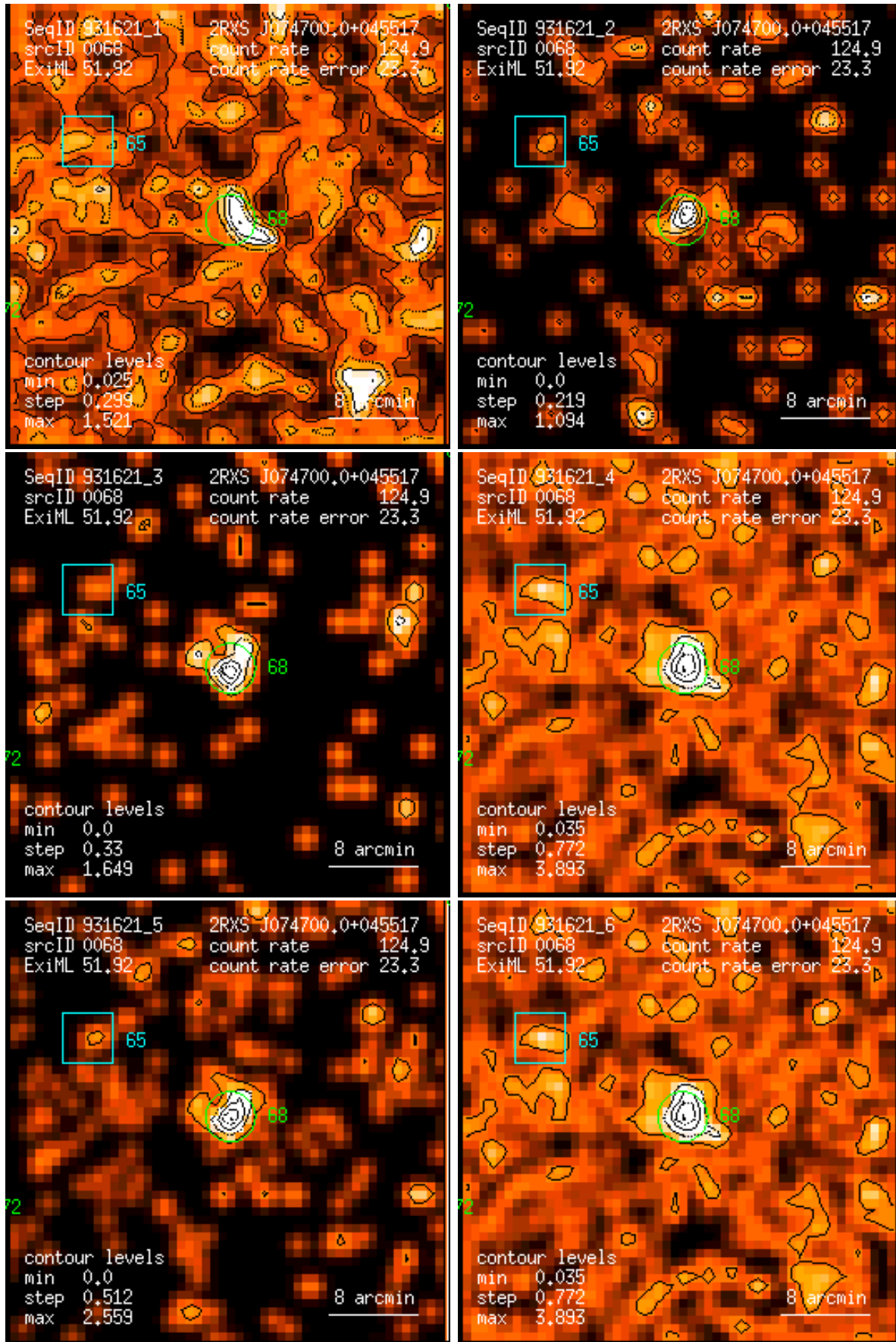
Figure 68: RASS 931621: detection 0068: band rate images, Gaussian filter: (1) PSPC channels 11 – 41, (2) 52 – 90, (3) 91 – 201, (4) 11 – 235, (5) 52 – 201, (6) 11 – 201. Broad band rates in counts/ks. Band rate contour levels in counts/ks/arcmin 2 .
