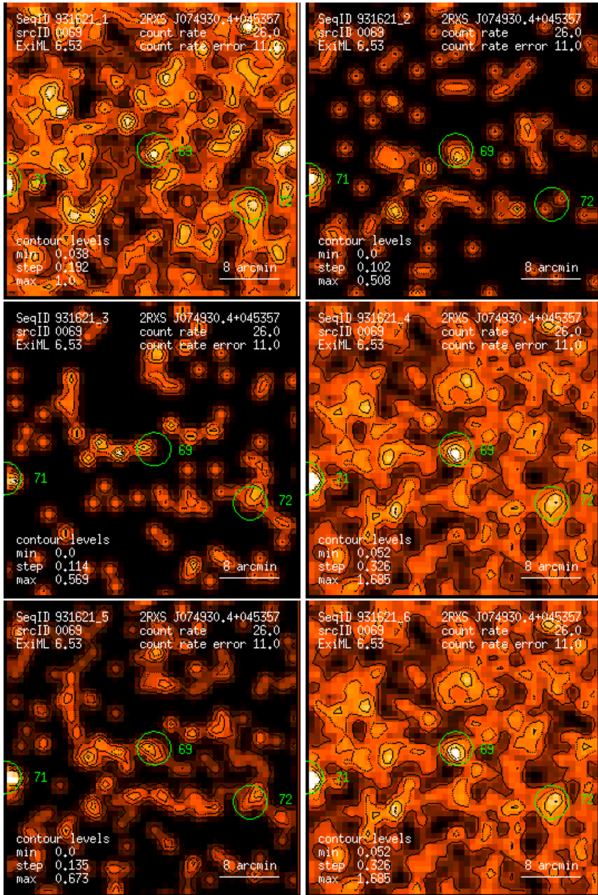
Figure 69: RASS 931621: detection 0069: band rate images, Gaussian filter: (1) PSPC channels 11 – 41, (2) 52 – 90, (3) 91 – 201, (4) 11 – 235, (5) 52 – 201, (6) 11 – 201. Broad band rates in counts/ks. Band rate contour levels in counts/ks/arcmin 2 .
