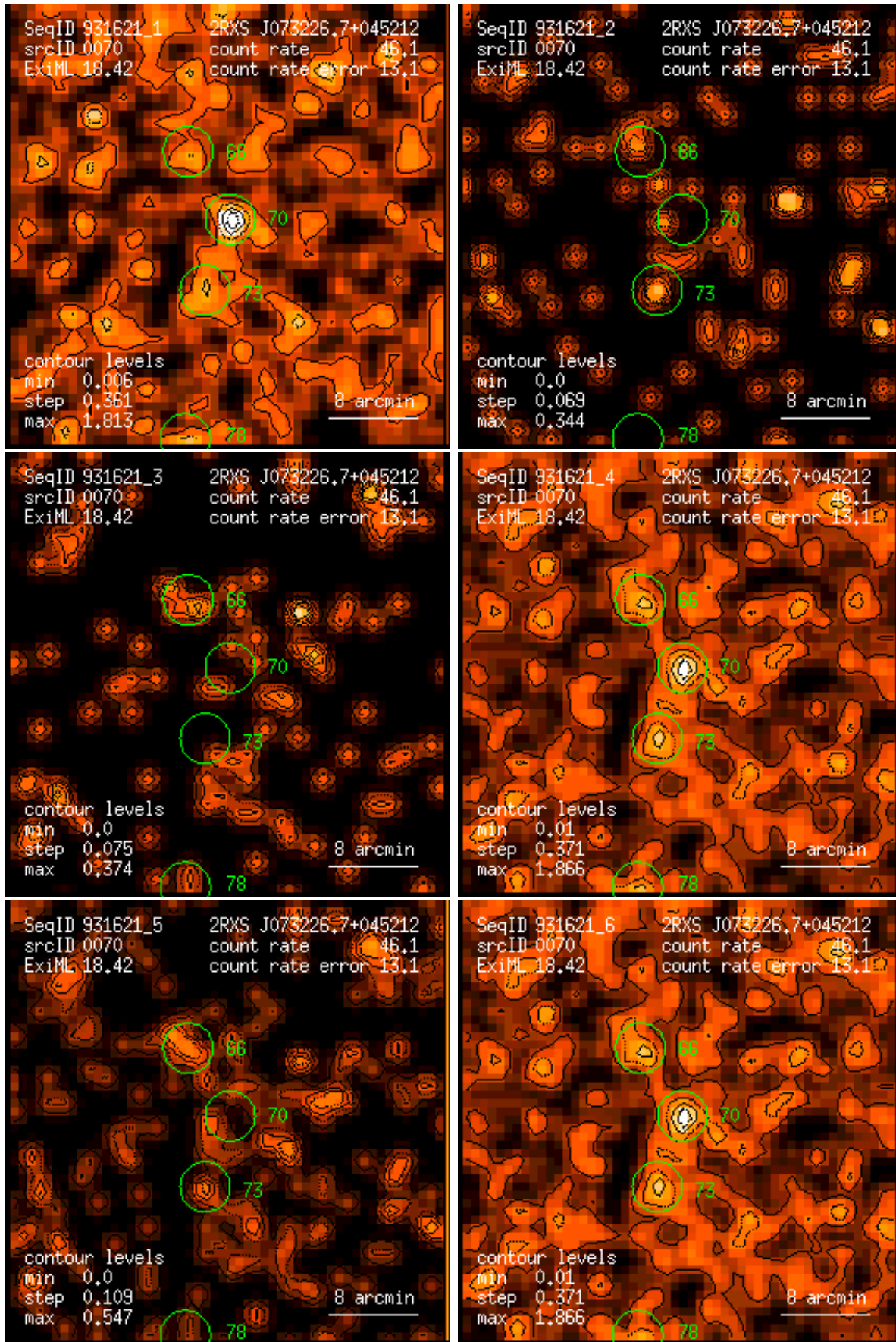
Figure 70: RASS 931621: detection 0070: band rate images, Gaussian filter: (1) PSPC channels 11 – 41, (2) 52 – 90, (3) 91 – 201, (4) 11 – 235, (5) 52 – 201, (6) 11 – 201. Broad band rates in counts/ks. Band rate contour levels in counts/ks/arcmin 2 .
