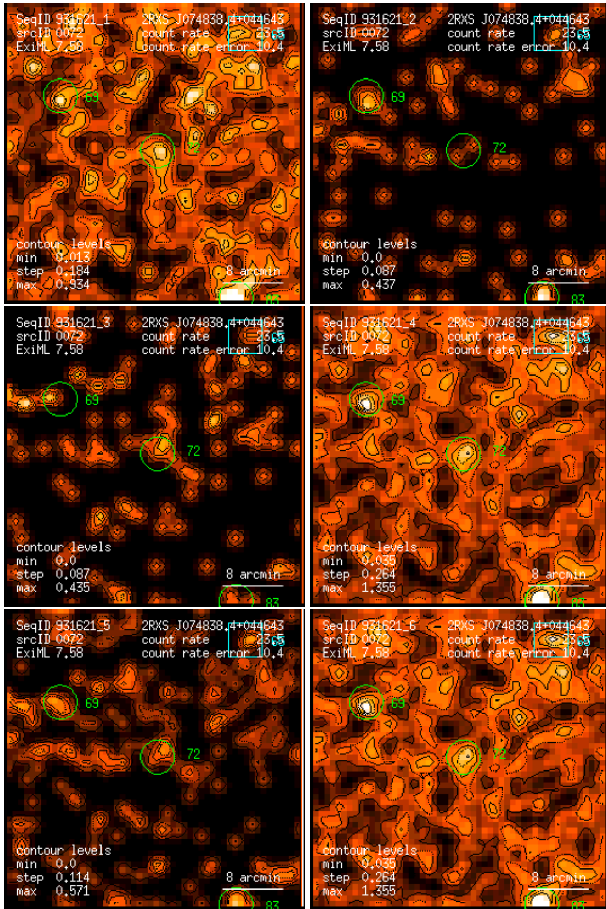
Figure 72: RASS 931621: detection 0072: band rate images, Gaussian filter: (1) PSPC channels 11 – 41, (2) 52 – 90, (3) 91 – 201, (4) 11 – 235, (5) 52 – 201, (6) 11 – 201. Broad band rates in counts/ks. Band rate contour levels in counts/ks/arcmin 2 .
