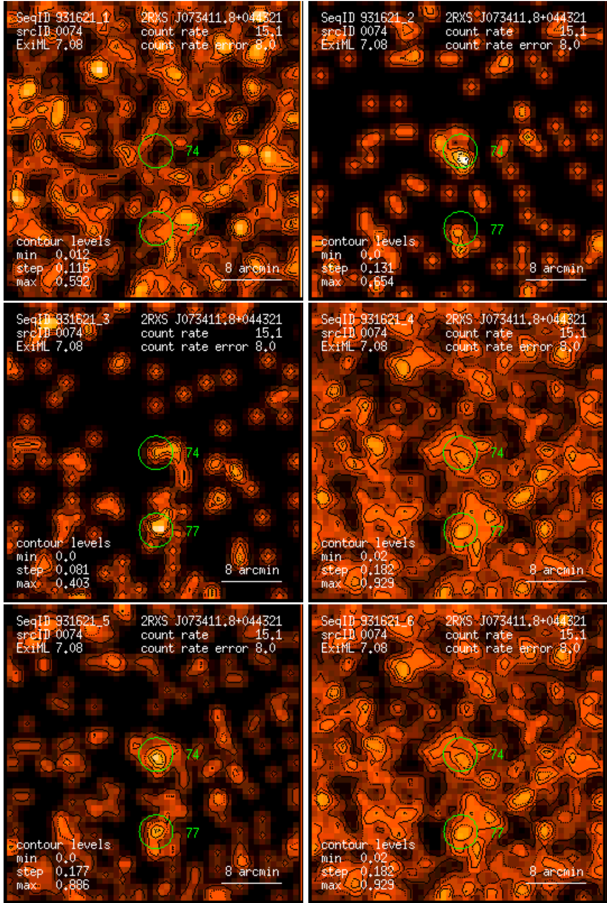
Figure 74: RASS 931621: detection 0074: band rate images, Gaussian filter: (1) PSPC channels 11 – 41, (2) 52 – 90, (3) 91 – 201, (4) 11 – 235, (5) 52 – 201, (6) 11 – 201. Broad band rates in counts/ks. Band rate contour levels in counts/ks/arcmin 2 .
