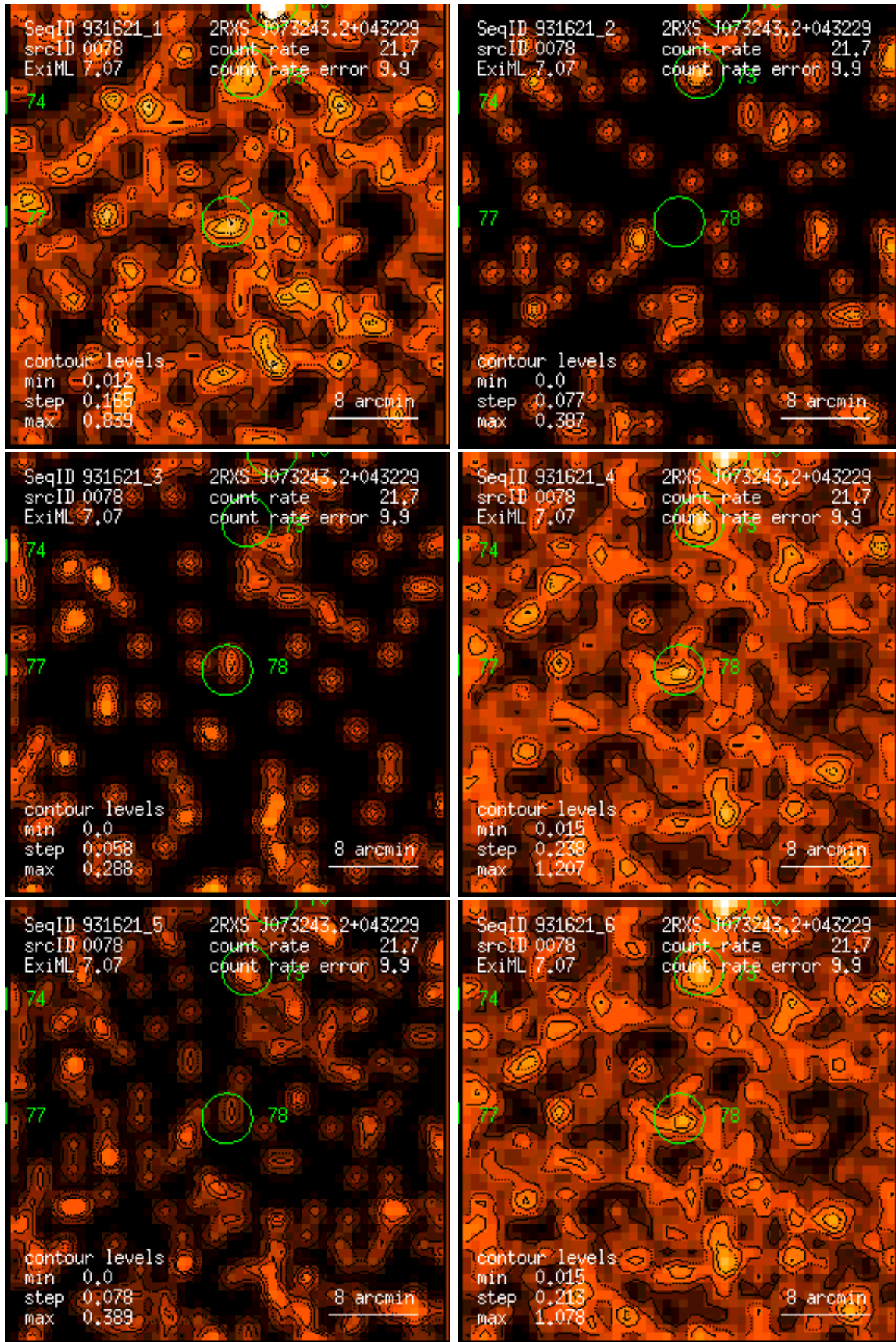
Figure 78: RASS 931621: detection 0078: band rate images, Gaussian filter: (1) PSPC channels 11 – 41, (2) 52 – 90, (3) 91 – 201, (4) 11 – 235, (5) 52 – 201, (6) 11 – 201. Broad band rates in counts/ks. Band rate contour levels in counts/ks/arcmin 2 .
