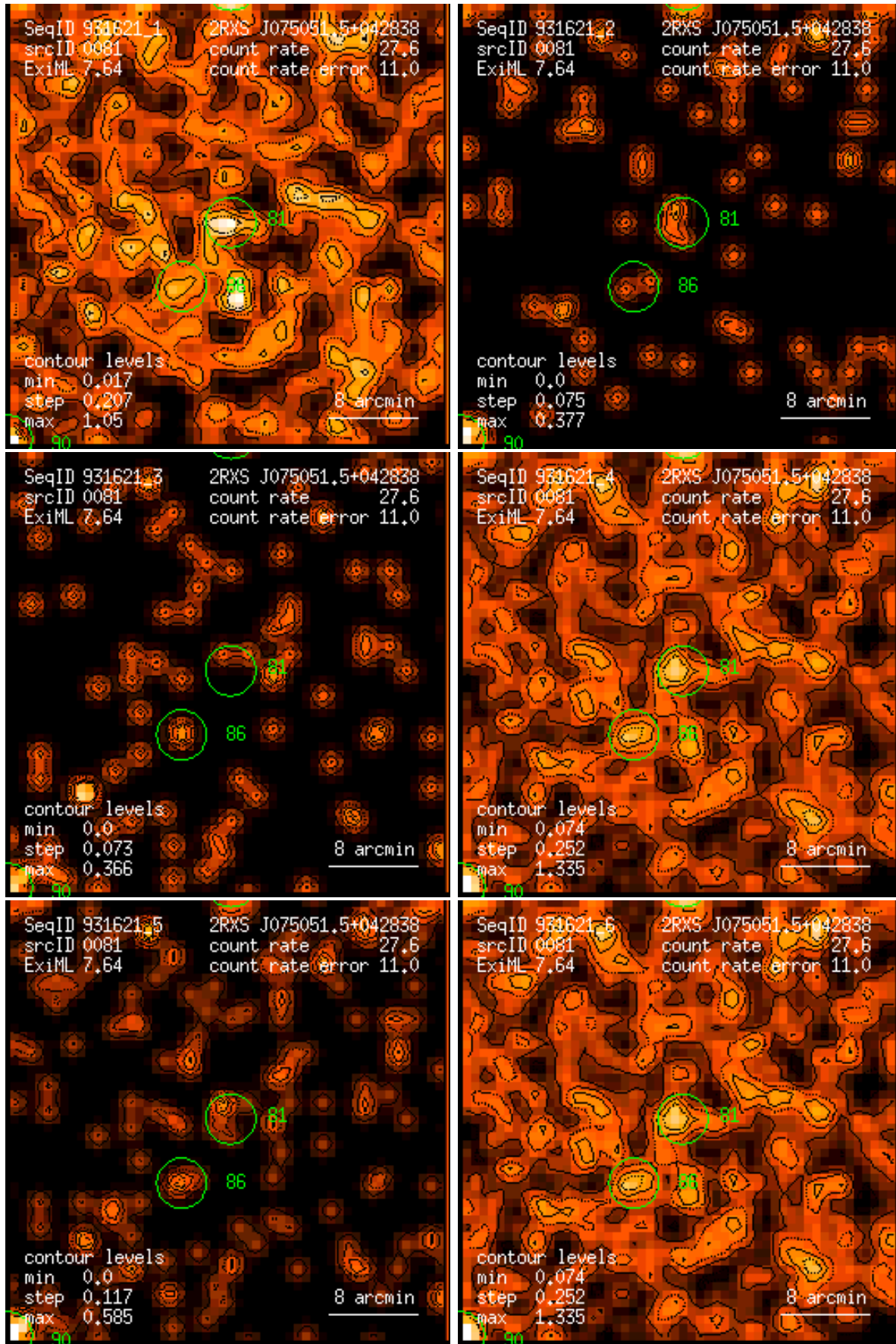
Figure 81: RASS 931621: detection 0081: band rate images, Gaussian filter: (1) PSPC channels 11 – 41, (2) 52 – 90, (3) 91 – 201, (4) 11 – 235, (5) 52 – 201, (6) 11 – 201. Broad band rates in counts/ks. Band rate contour levels in counts/ks/arcmin 2 .
