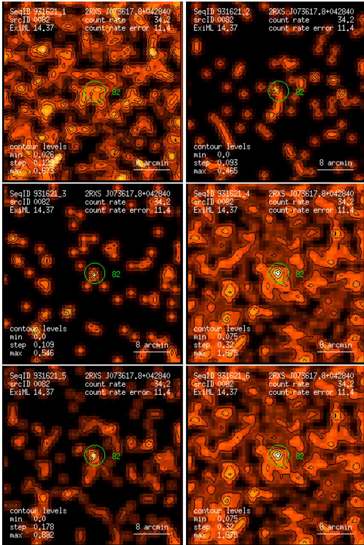
Figure 82: RASS 931621: detection 0082: band rate images, Gaussian filter: (1) PSPC channels 11 – 41, (2) 52 – 90, (3) 91 – 201, (4) 11 – 235, (5) 52 – 201, (6) 11 – 201. Broad band rates in counts/ks. Band rate contour levels in counts/ks/arcmin 2 .
