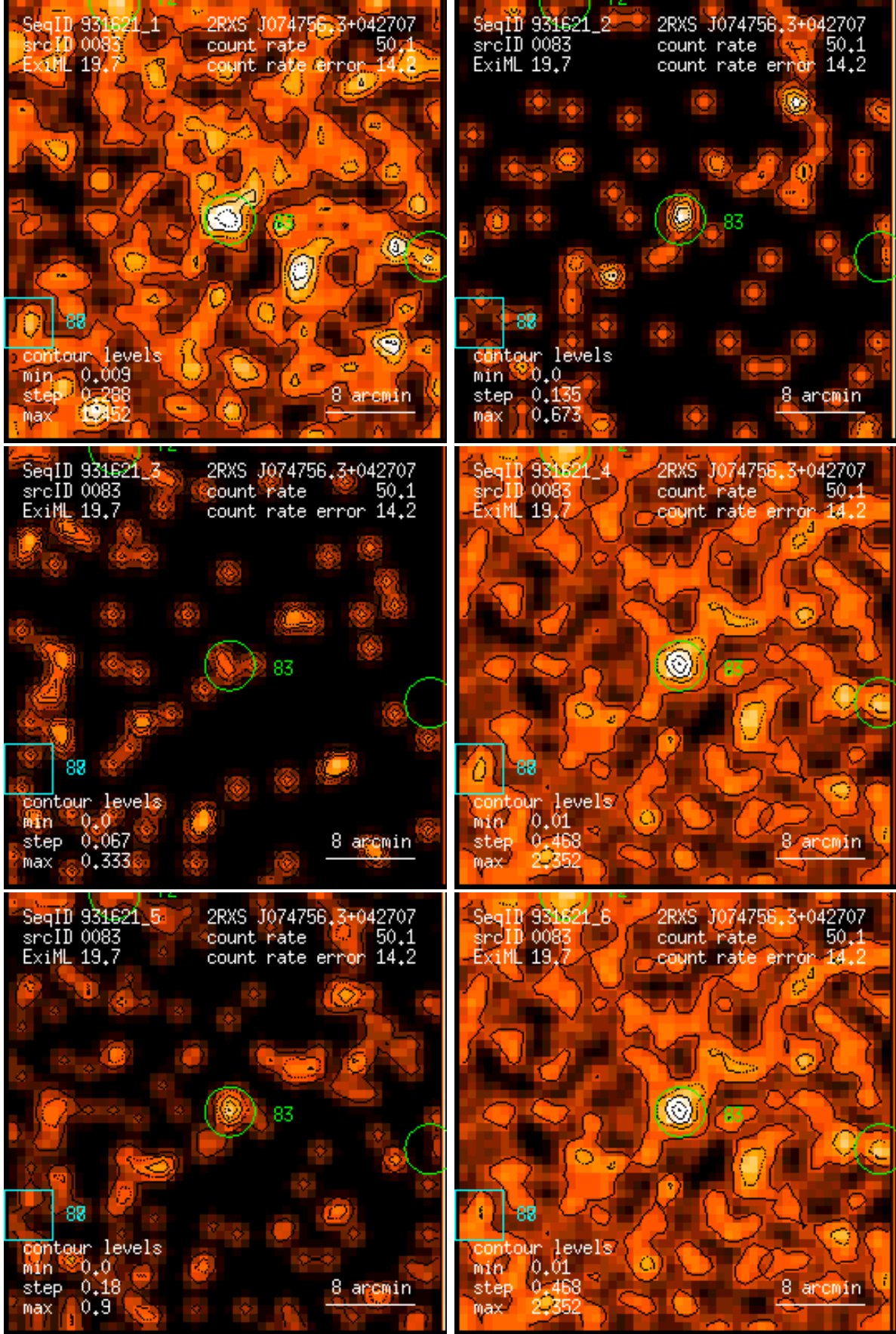
Figure 83: RASS 931621: detection 0083: band rate images, Gaussian filter: (1) PSPC channels 11 – 41, (2) 52 – 90, (3) 91 – 201, (4) 11 – 235, (5) 52 – 201, (6) 11 – 201. Broad band rates in counts/ks. Band rate contour levels in counts/ks/arcmin 2 .
