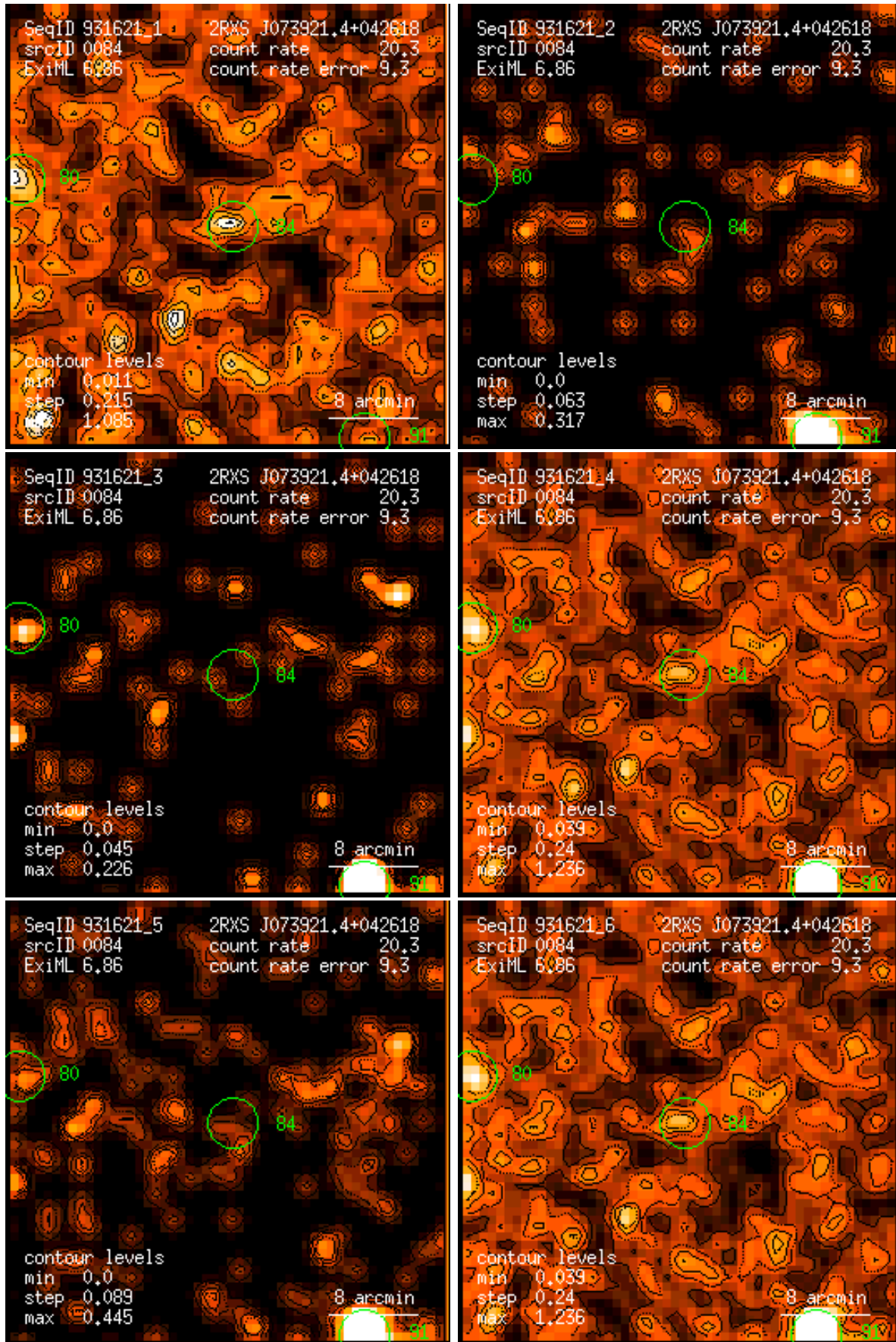
Figure 84: RASS 931621: detection 0084: band rate images, Gaussian filter: (1) PSPC channels 11 – 41, (2) 52 – 90, (3) 91 – 201, (4) 11 – 235, (5) 52 – 201, (6) 11 – 201. Broad band rates in counts/ks. Band rate contour levels in counts/ks/arcmin 2 .
