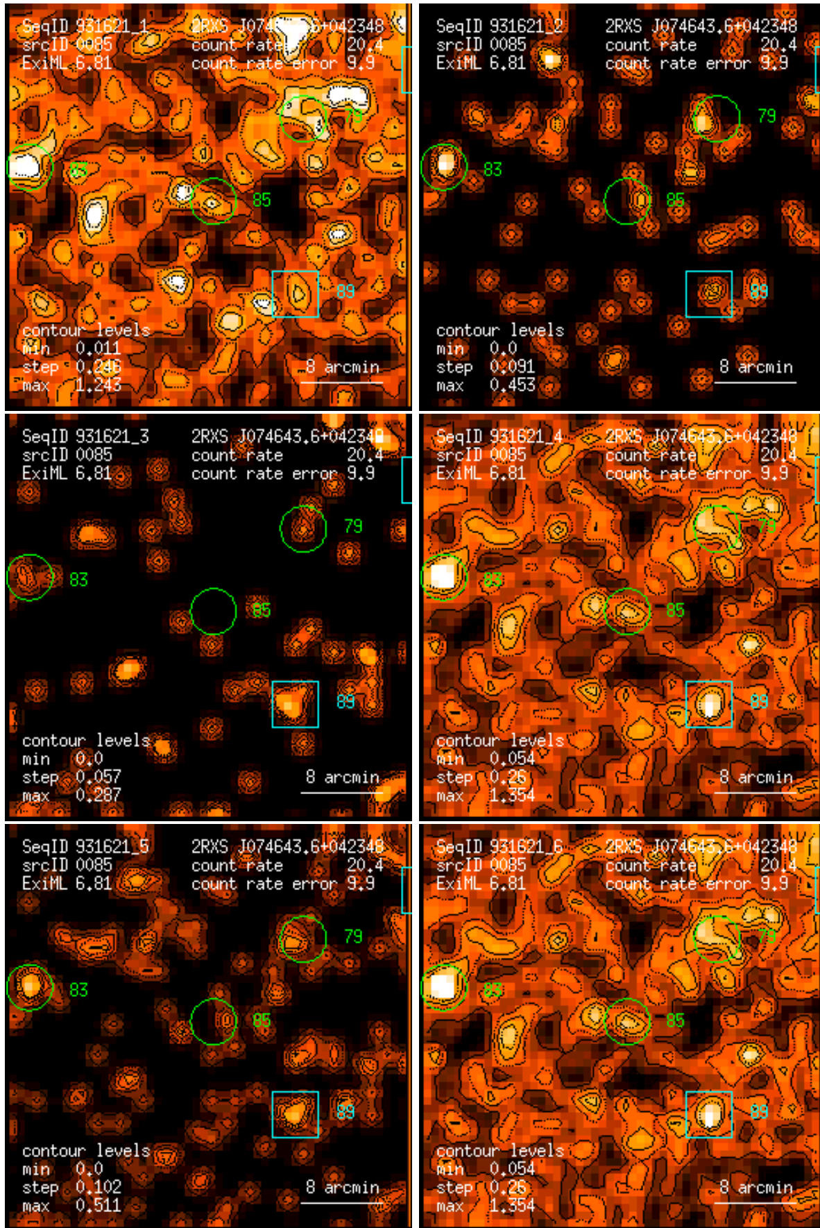
Figure 85: RASS 931621: detection 0085: band rate images, Gaussian filter: (1) PSPC channels 11 – 41, (2) 52 – 90, (3) 91 – 201, (4) 11 – 235, (5) 52 – 201, (6) 11 – 201. Broad band rates in counts/ks. Band rate contour levels in counts/ks/arcmin 2 .
