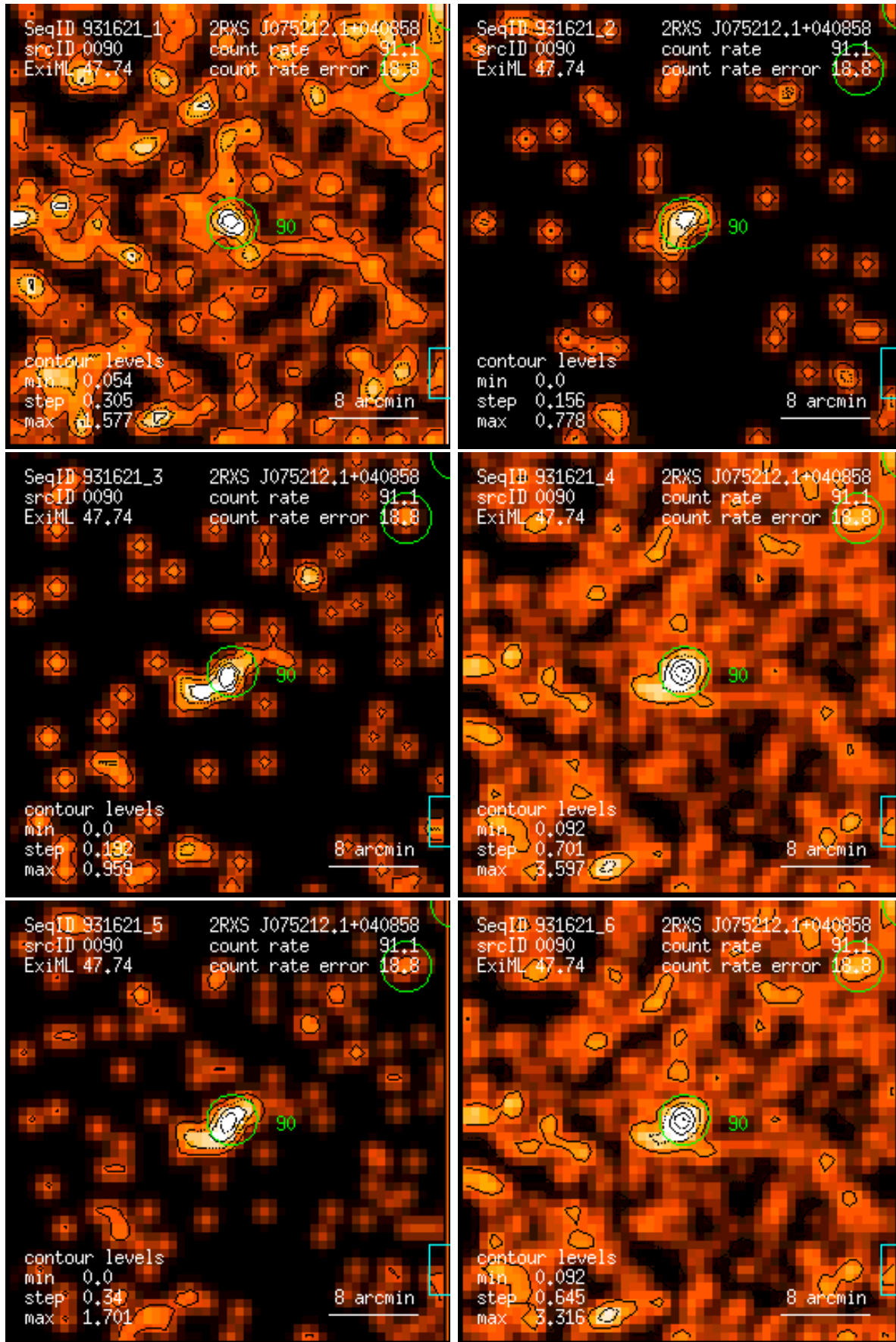
Figure 90: RASS 931621: detection 0090: band rate images, Gaussian filter: (1) PSPC channels 11 – 41, (2) 52 – 90, (3) 91 – 201, (4) 11 – 235, (5) 52 – 201, (6) 11 – 201. Broad band rates in counts/ks. Band rate contour levels in counts/ks/arcmin 2 .
