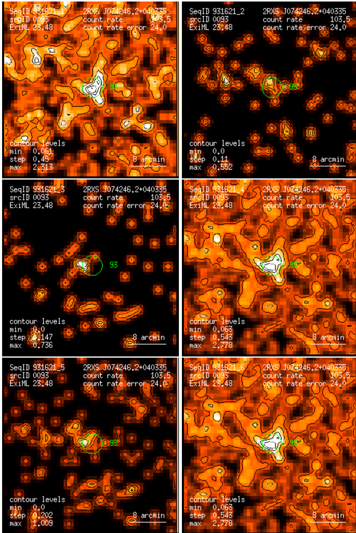
Figure 93: RASS 931621: detection 0093: band rate images, Gaussian filter: (1) PSPC channels 11 – 41, (2) 52 – 90, (3) 91 – 201, (4) 11 – 235, (5) 52 – 201, (6) 11 – 201. Broad band rates in counts/ks. Band rate contour levels in counts/ks/arcmin 2 .
