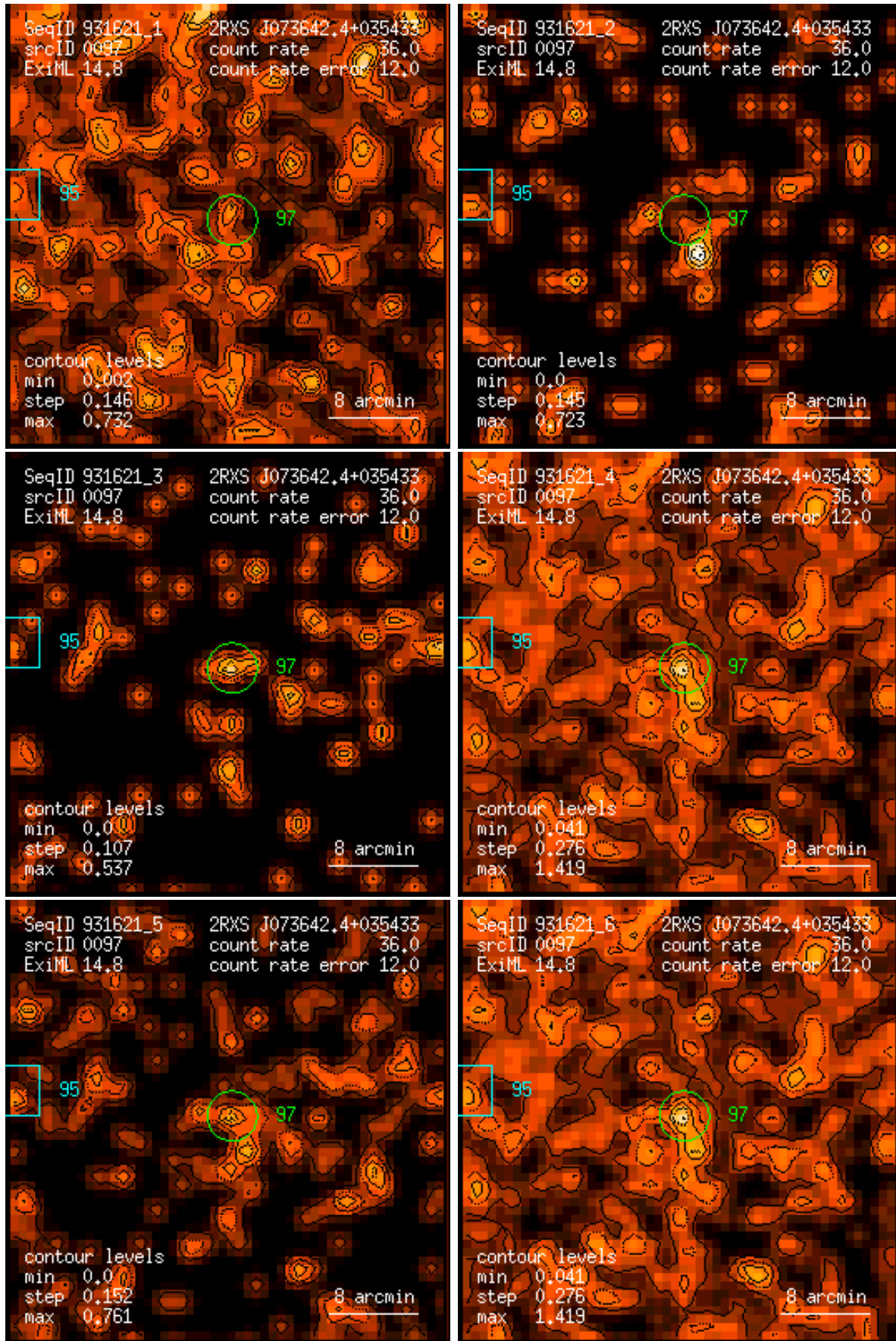
Figure 97: RASS 931621: detection 0097: band rate images, Gaussian filter: (1) PSPC channels 11 – 41, (2) 52 – 90, (3) 91 – 201, (4) 11 – 235, (5) 52 – 201, (6) 11 – 201. Broad band rates in counts/ks. Band rate contour levels in counts/ks/arcmin 2 .
