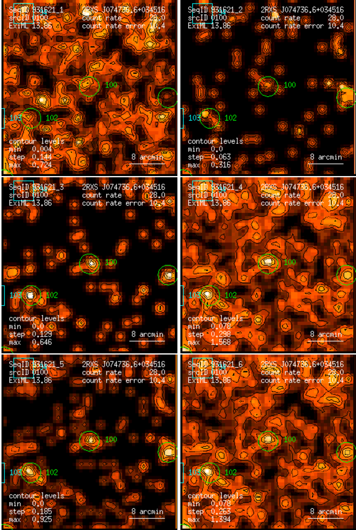
Figure 100: RASS 931621: detection 0100: band rate images, Gaussian filter: (1) PSPC channels 11 – 41, (2) 52 – 90, (3) 91 – 201, (4) 11 – 235, (5) 52 – 201, (6) 11 – 201. Broad band rates in counts/ks. Band rate contour levels in counts/ks/arcmin 2 .
