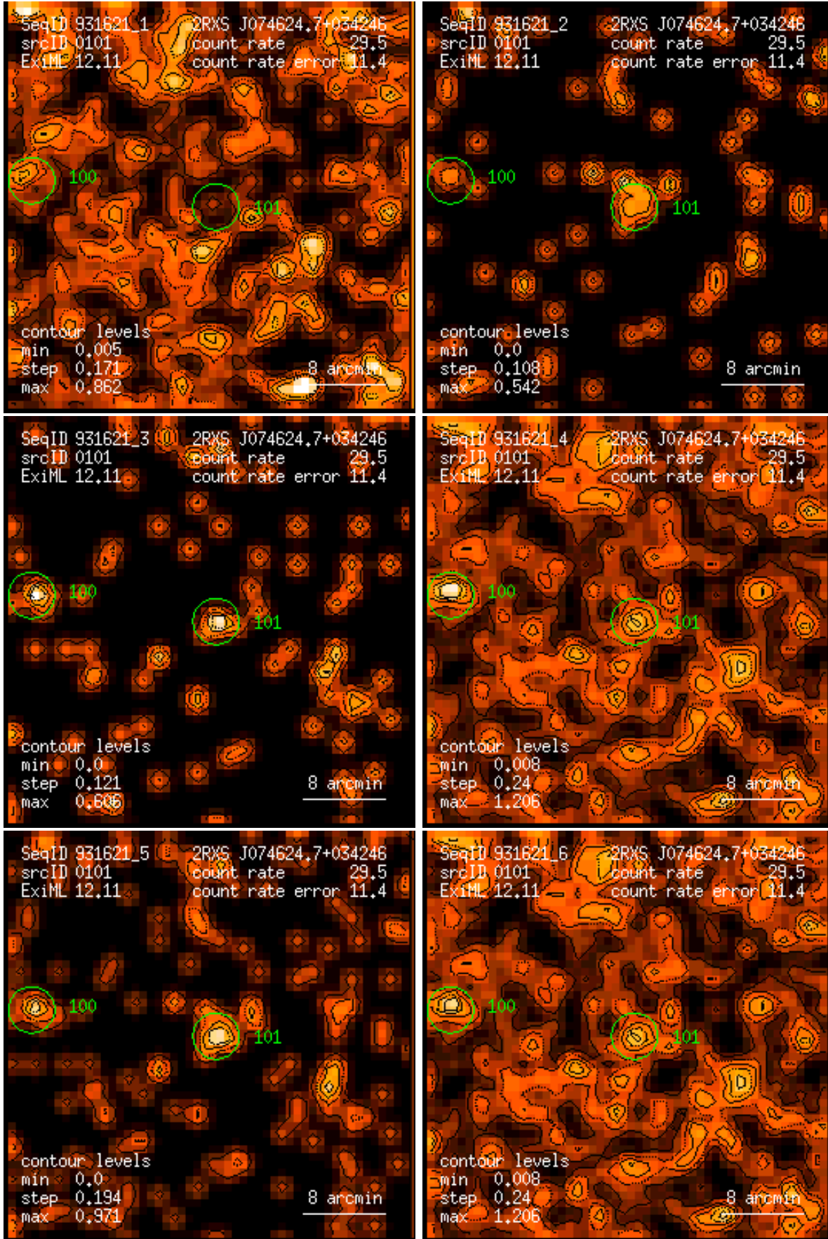
Figure 101: RASS 931621: detection 0101: band rate images, Gaussian filter: (1) PSPC channels 11 – 41, (2) 52 – 90, (3) 91 – 201, (4) 11 – 235, (5) 52 – 201, (6) 11 – 201. Broad band rates in counts/ks. Band rate contour levels in counts/ks/arcmin 2 .
