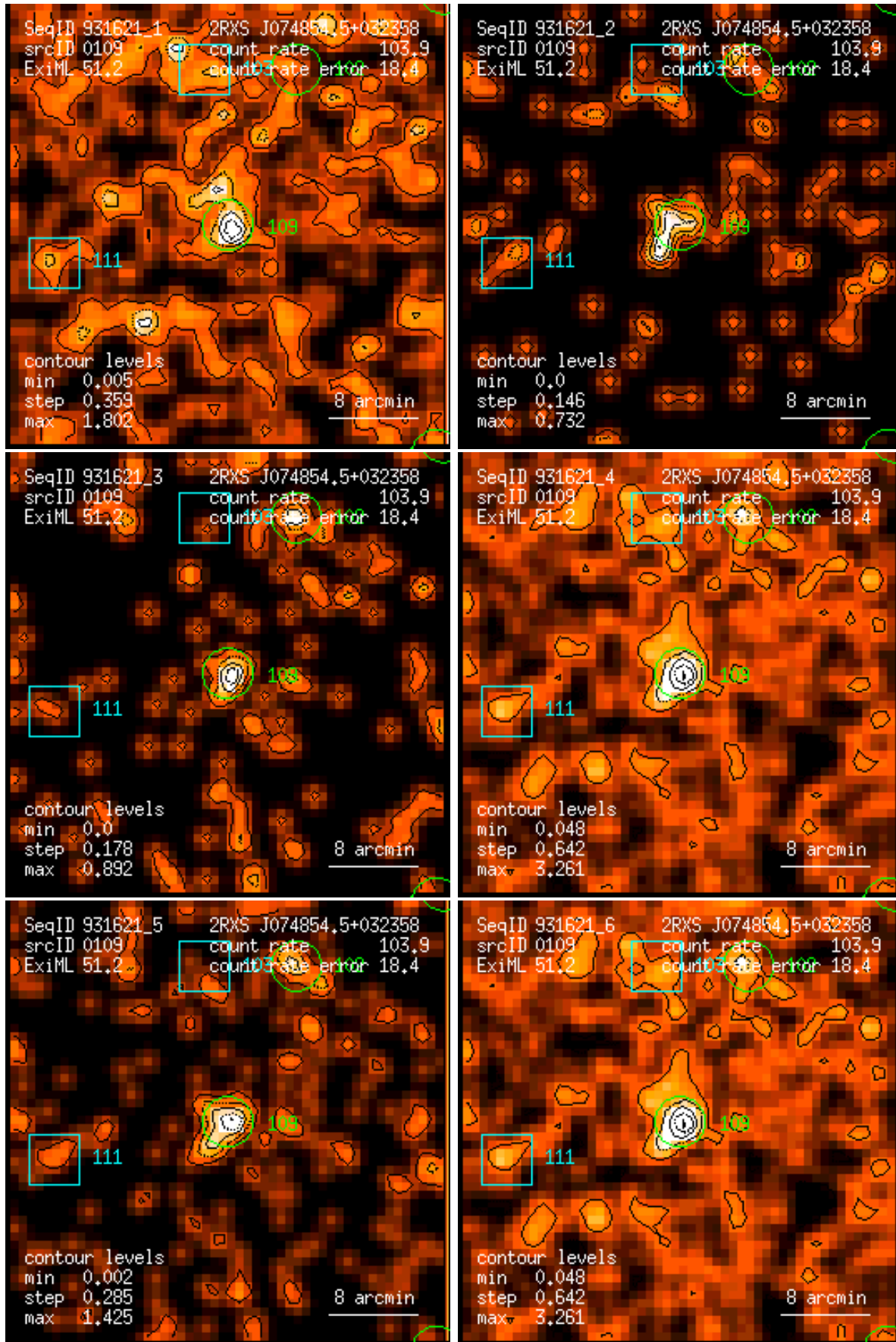
Figure 109: RASS 931621: detection 0109: band rate images, Gaussian filter: (1) PSPC channels 11 – 41, (2) 52 – 90, (3) 91 – 201, (4) 11 – 235, (5) 52 – 201, (6) 11 – 201. Broad band rates in counts/ks. Band rate contour levels in counts/ks/arcmin 2 .
